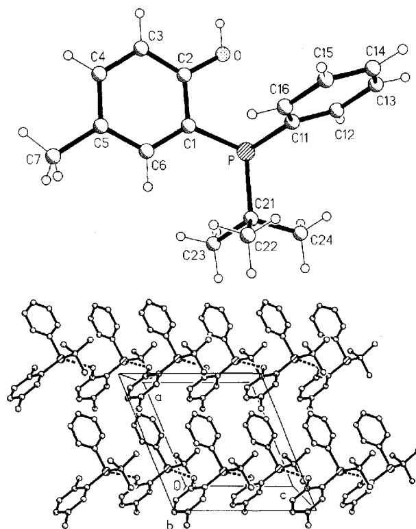
Figure 4. Crystal and molecular structure of 5d ; selected distances [pm] and angles [\circ] : \text{P}-\text{C}1 183.1(2), \text{P}-\text{C}11 183.2(2), \text{P}-\text{C}21 187.6(2), \text{O}-\text{C}2 136.5(2); \text{C}1-\text{P}-\text{C}11 101.80(7) , \text{C}1-\text{P}-\text{C}21 110.00(7) , \text{C}11-\text{P}-\text{C}21 103.57(7) , \text{P}-\text{C}1-\text{C}2 113.91(11) , \text{O}-\text{C}2-\text{C}1 116.01(13) , \text{P}-\text{C}11-\text{C}12 117.86(12) , \text{P}-\text{C}11-\text{C}16 123.39(12) ; \text{P}\cdots\text{O} 278.5(1); intermolecular (x, 1/2 - y, 1/2 + z) \text{P}\cdots\text{H}-\text{O} see text
