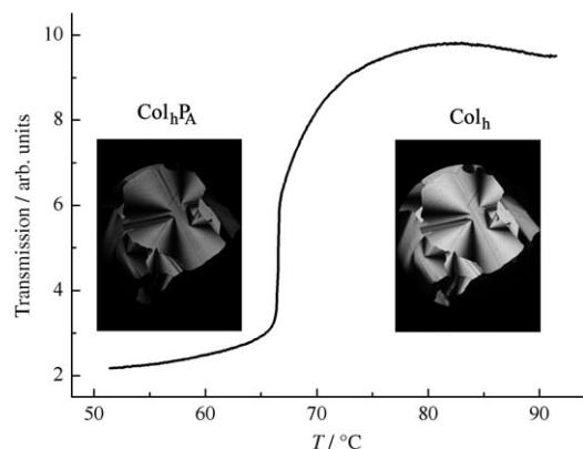
Figure 1. Light transmission through the circular domain, measured as a function of temperature for compound 9b in three micron cell, reveals a decrease of optical birefringence at Col h –Col h P A phase transition. In the inset the texture of Col h and Col h P A phases.
