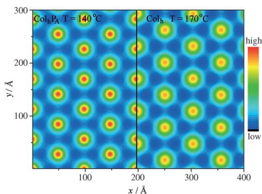
Figure 2. Electron density maps obtained in the plane perpendicular to the column axis in Col h and Col h P A phases for compound 1a . The relative intensities of XRD signals used for electron density calculations were, in Col h phase: I_{10}/I_{11}/I_{20} 130:1:2; in Col h P A : I_{10}/I_{11}/I_{20}/I_{21} 130:10:10:2.
