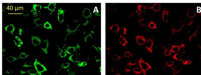
Figure 5. Confocal microscopy images (A: \lambda_{\text{exc}} = 488 nm; B: \lambda_{\text{exc}} = 561 nm) of human breast cancer cells MCF7 with fluorophore 11 .
