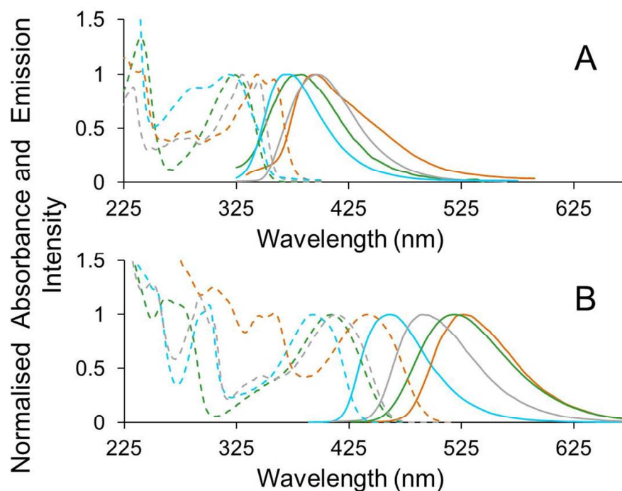
Figure 1. Absorption (dashed plot) and emission spectra (continuous plot) of ligands (A) and complexes (B) in \text{CH}_3\text{CN} ( 2 \times 10^{-5} \text{M} ). 6&10 , grey; 7&11 , orange; 8&12 , blue; 9&13 , green.
