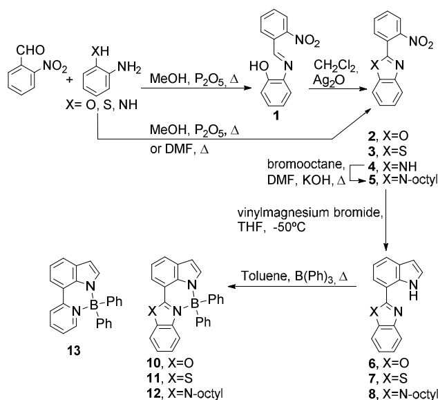
Scheme 1. Synthetic route to ligands and organoboron complexes.
