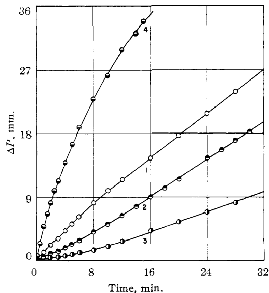
Fig. 3.—Pressure increase during the decomposition of 200 mm. of methyl n -butyl ketone at 450°: ○, pure ketone; ●, packed bulb (other curves from unpacked bulb); ◐, 105 mm. of propylene added; ●, 1% ethylene oxide and 99% ketone.
