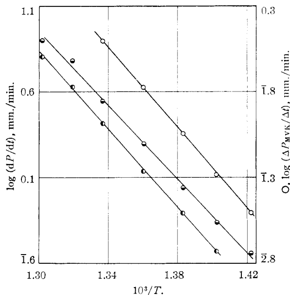
Fig. 5.—Variation of rate with temperature: \bullet , (dP/dt)_0 , initial rate of pressure rise; \bullet , (dP/dt)_{0.10} , rate of pressure rise after \sim 10\% pressure increase; \circ , (\Delta P_{MVK}/\Delta t) , initial rate of appearance of methyl vinyl ketone.
