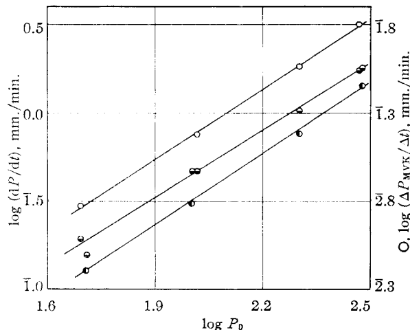
Fig. 4.—Change in rate with initial pressure, P_0 : \circ , (dP/dt)_0 , initial rate of pressure rise; \bullet , (dP/dt)_{0.06} , rate of pressure rise after \sim 6\% pressure increase; \circ , (\Delta P_{MVK}/\Delta t) , average rate of build-up of methyl vinyl ketone during the first 8 min. Each point showing the rate of pressure rise at 200 mm. represents the average of three values.
