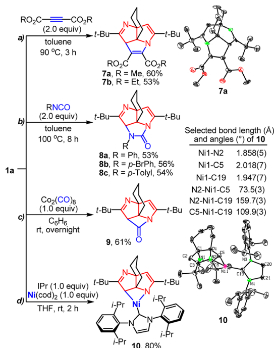
Scheme 4. Insertions into the Weakened C–N Bonds
