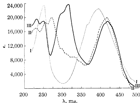
Fig. 1.—Absorption spectra in absolute ethanol of compounds I, II and III.
