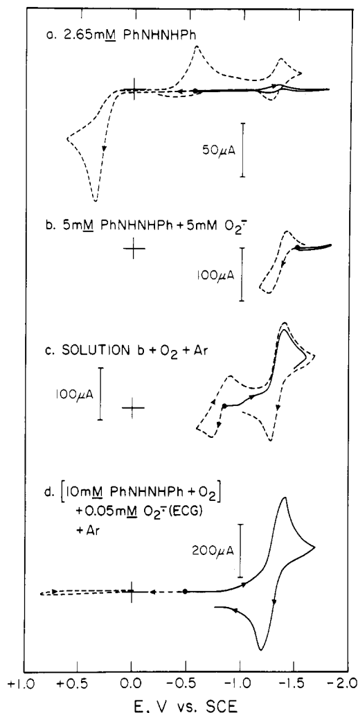
Figure 1. Cyclic voltammograms in dimethyl sulfoxide (0.1 M tetraethylammonium perchlorate) for (a) 1,2-diphenylhydrazine (PhNHNHPh), (b) an equimolar mixture of PhNHNHPh and O_2^{\bullet-} (electrogenerated) in an argon atmosphere, (c) solution b after exposure to O_2 (1 atm) for 3 min followed by a 5-min purge with argon, and (d) 10 mM PhNHNHPh in an O_2 (1 atm)-saturated solution after the in situ electrogeneration of 0.05 mM O_2^{\bullet-} (1 min) followed by a 5-min purge with argon. Measurements were made with a platinum electrode (area, 0.23 \text{ cm}^2 ) at a scan rate of 0.1 \text{ V s}^{-1} .
