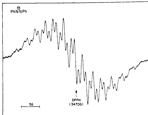
Figure 3. ESR spectrum at 77 K for the product species (10 mM) from the 1:1 combination of PhNHNHPh with O 2 •- [(Me 4 N)O 2 ] in MeCN. This spectrum is identical with that for the product (PhN • -NPh) from the one-electron controlled-potential electrolytic reduction of 10 mM PhN=NPh.
