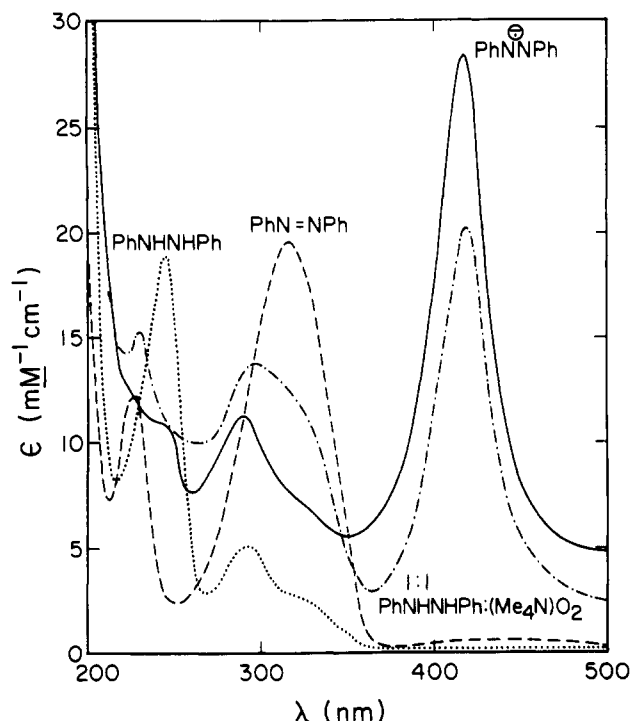
Figure 2. UV-vis absorption spectra in MeCN for 5 mM 1,2-diphenylhydrazine (PhNHNHPh), 5 mM azobenzene (PhN=NPh), 5 mM PhN • -NPh (from the one-electron controlled-potential electrolytic reduction of 5 mM PhN=NPh), and the product solution from the 1:1 combination of PhNHNHPh and (Me 4 N)O 2 (each 5 mM before reaction). The latter spectrum is normalized with respect to \epsilon on the assumption that a single 5 mM product species is formed.
