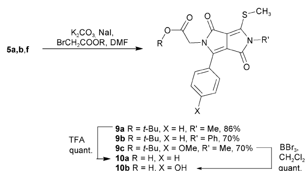
Scheme 2 N -Alkylation of SDPPs 5a, b and f .
