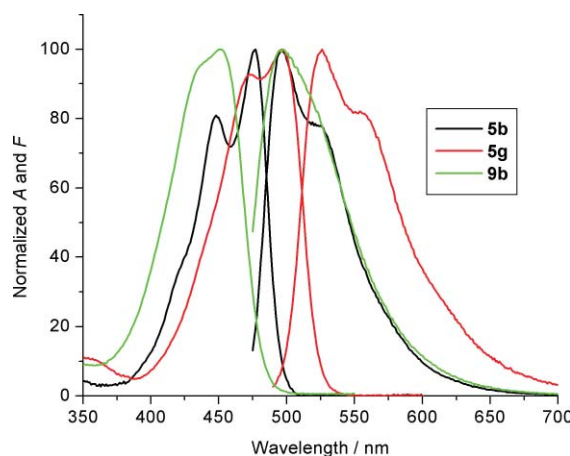
Fig. 1 Normalized absorption ( A ) and fluorescence emission ( F ) spectra (excitation at 470 nm) of 5b (black) and 5g (red) in toluene and 9b (green) in methanol.
