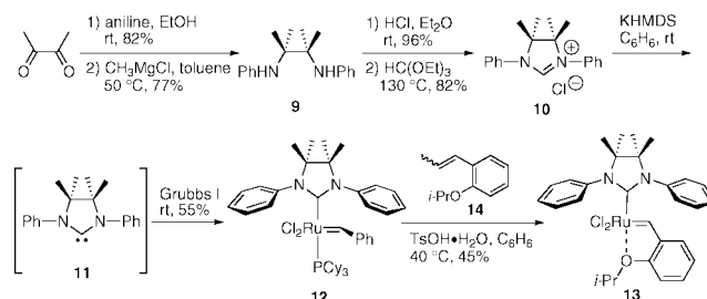
Scheme 1. Synthesis of Ruthenium Complex 13
