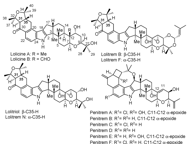
Figure 1. Selected tremorgenic indole natural products.
