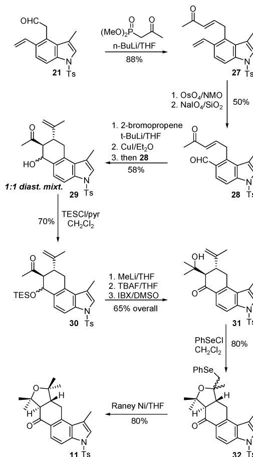
Scheme 5. Successful Synthesis of the Western Half of Lolicine A
