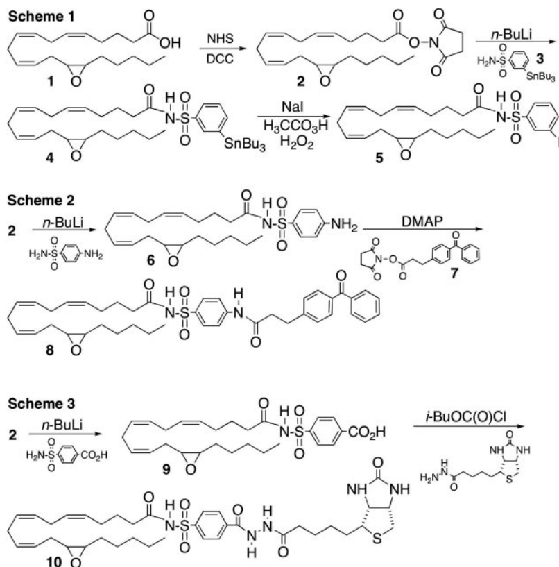
Fig. 1. Synthesis of 14,15-EET-sulfonamides in Schemes 1, 2, and 3.
