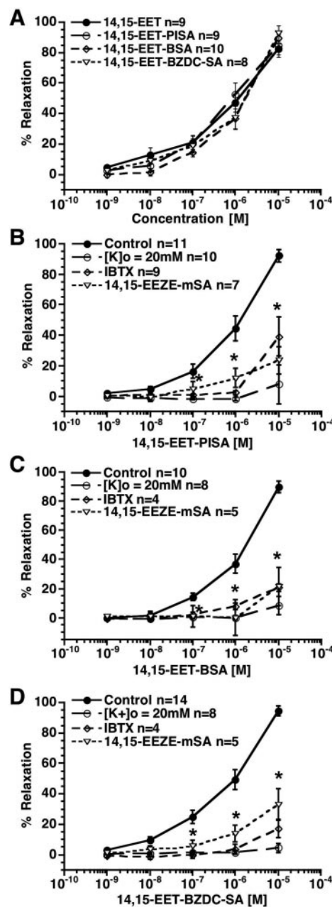
Fig. 3. Effects of 14,15-EET and 14,15-EET-sulfonamides on vascular tone of U46619 precontracted bovine coronary arteries. A, relaxations to 14,15-EET, 14,15-EET-PISA, 14,15-EET-BSA, and 14,15-EET-BZDC-SA. B to D, effects of the BK_{Ca} channel inhibitor, IBTX (100 nM); the EET antagonist, 14,15-EEZE-mSA (10 \mu M); or increased extracellular K^+ (20 mM) on 14,15-EET-PISA (B), 14,15-EET-BSA (C), and 14,15-EET-BZDC-SA (D) relaxations. *, significantly different from control, P < 0.05 .
