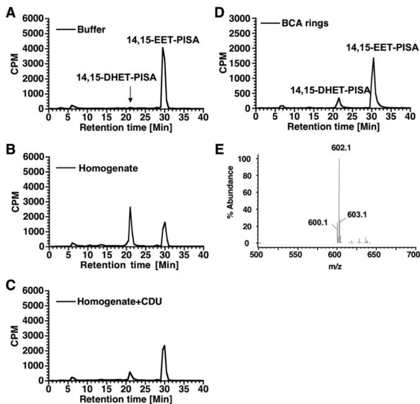
Fig. 4. Metabolism of 14,15-EET- \text{P}^{125}\text{ISA} by BCA homogenate and arterial rings. A to C, HPLC chromatograms of extracted 14,15-EET- \text{P}^{125}\text{ISA} metabolites after incubation with buffer, BCA homogenate ( 500 \mu\text{g} ) in the presence or absence of CDU ( 1 \mu\text{M} ) for 30 min at 30^\circ\text{C} , respectively. D, HPLC chromatogram of extracted 14,15-EET- \text{P}^{125}\text{ISA} metabolites after incubation with arterial rings for 15 min at 37^\circ\text{C} . E, Negative ion electrospray ionization MS spectrum of 14,15-EET-PISA metabolite (peak 21).
