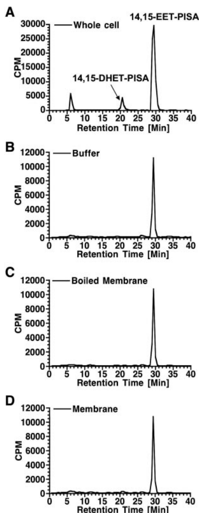
Fig. 5. Metabolism of 14,15-EET- P^{125} ISA by U937 cells and U937 membrane protein. A, 14,15-EET- P^{125} ISA (35 nM) was incubated with intact U937 cells (800,000 cells) for 15 min at 37°C. B to D, 14,15-EET- P^{125} ISA (1 nM) was incubated with buffer (B), boiled U937 membrane protein (C), or U937 membrane protein (50 \mu g, D) for 15 min at 4°C. HPLC chromatograms of extracted 14,15-EET- P^{125} ISA metabolites from the incubations were shown.
