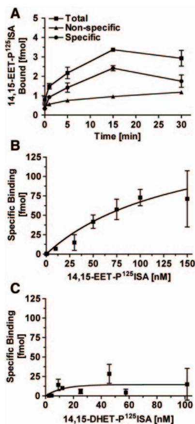
Fig. 6. 14,15-EET- P^{125} ISA binding to U937 membrane protein. A, time course of 14,15-EET- P^{125} ISA binding. 14,15-EET- P^{125} ISA (1 nM) was incubated with 50 \mu g of protein at 4°C for various time (1–30 min). n = 2 . B, concentration-dependent 14,15-EET- P^{125} ISA binding. Increasing concentrations of 14,15-EET- P^{125} ISA (0.1–150 nM) were incubated with 50 \mu g of protein at 4°C for 15 min. n = 2 –7. C, 14,15-DHET- P^{125} ISA binding to U937 membranes. Increasing concentrations of 14,15-DHET- P^{125} ISA (2.5–100 nM) were incubated with 50 \mu g of protein at 4°C for 15 min. n = 2 –3.
