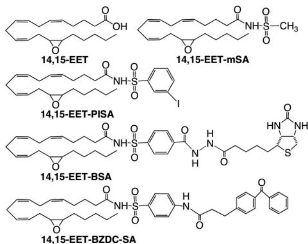
Fig. 2. Structures of 14,15-EET and 14,15-EET-sulfonamides.
