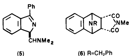
Scheme 2. (i) e.g. \text{CH}_2=\text{NMe}_2\text{Cl}^+ , \text{CH}_3\text{CN} (ii) 1, \text{H}^+ ; or self condensation (iii) -\text{2H} (air) (iv) 5, \text{H}^+ ; 44% (v) 1-formyl-3-phenylisoindole, \text{H}^+ ; 63% (yields not optimised).
