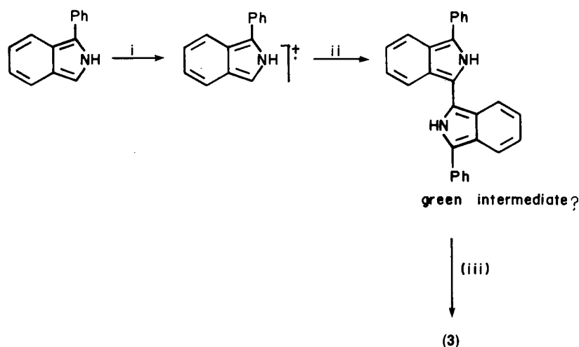
Scheme 1. (i) \text{H}_2\text{NO}_2^+ , -\text{e} (ii) 1-phenylisoindole, -2\text{H}^+ , -\text{e} or 2\text{x} , -2\text{H}^+ (iii) air, -2\text{H} .
