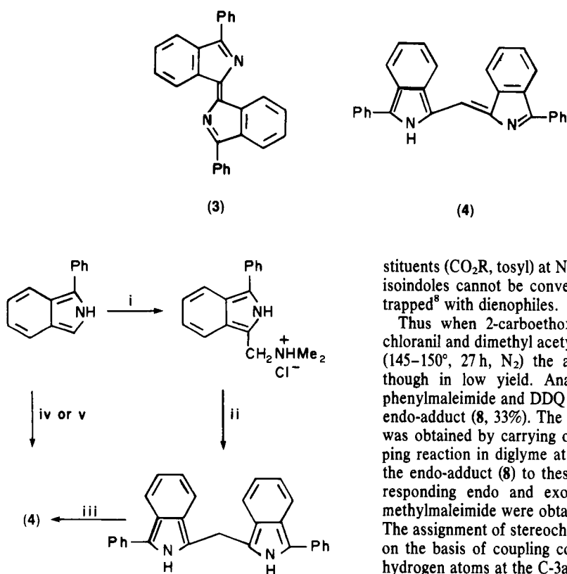
Scheme 2. (i) e.g. \text{CH}_2=\text{NMe}_2\text{Cl}^+ , \text{CH}_3\text{CN} (ii) 1, \text{H}^+ ; or self condensation (iii) -\text{2H} (air) (iv) 5, \text{H}^+ ; 44% (v) 1-formyl-3-phenylisoindole, \text{H}^+ ; 63% (yields not optimised).
