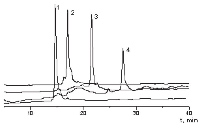
Fig. 1 Reversed-phase HPLC traces of crude oligonucleotide 2'-conjugates: (1) oligonucleotide II ; (2) conjugate II.20 ; (3) conjugate II.17 ; (4) conjugate II.14 . For HPLC conditions, see Experimental section.
