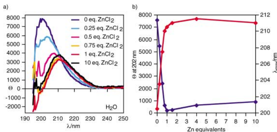
Fig. 5. Titration of \beta -peptide 2 with \text{ZnCl}_2 and determination of the complex stoichiometry. a) The intensity and the wavelength of the CD band change rapidly when addition of \text{ZnCl}_2 approaches equimolar amounts (red curves). Upon addition of excess \text{ZnCl}_2 (up to 10 equiv.), the CD curve remains unchanged (black curve). b) Plotting the molar ellipticity, observed at 202 nm (blue), and the shift of the wavelength of the maximum of each curve (red) vs. the number of equiv. \text{Zn}^{2+} , it is possible to conclude that the complex stoichiometry is 1:1 (peptide 0.2 mM in 50 mM Tris buffer).
