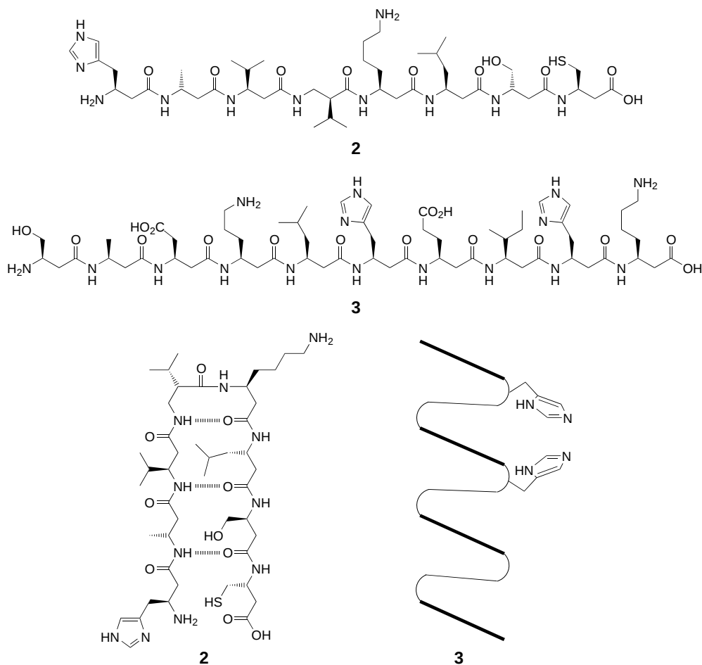
Fig. 2. Formulae and schematic presentations of the \beta -peptides 2 and 3 . \beta -Octapeptide 2 in a possible hairpin conformation with three trans -strand H-bonds, and \beta^3\text{hCys} and \beta^3\text{hHis} in the right position for metal-ion binding. \beta -Decapeptide 3 in a 3_{14} -helical conformation where two \beta^3\text{hHis} , as well as \beta^3\text{hOrn} , \beta^3\text{hLys} and \beta^3\text{hGlu} are placed in i and i + 3 positions, respectively. The two 1 H -imidazol-4-yl groups in juxtaposition on the helix should complex \text{Zn}^{2+} . At slightly acidic pH, two salt bridges should stabilize the helix.
