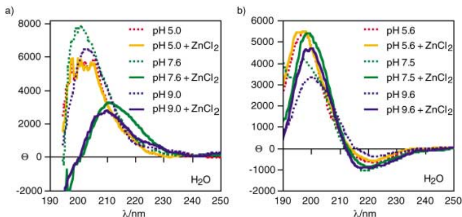
Fig. 4. Normalized CD spectra of \beta -octapeptide 2 and \beta -decapeptide 3 in \text{H}_2\text{O} at different pH values, with and without \text{ZnCl}_2 . a) The CD spectrum of \beta -peptide 2 at pH 7.6 looks similar to the one in MeOH (green, dotted line). Upon addition of \text{Zn}^{2+} ions, the \lambda_{\text{max}} is shifted by ca. 10 nm, and the intensity of the CD band decreases to half the value (green, solid line). The same behavior is observed at pH 9 (blue, dotted and solid lines, resp.), but not at pH 5.0 (red and orange, dotted and solid lines, resp.), probably because the donor 1 H -imidazol-4-yl group of 2 is protonated and no longer available for coordination to the metal (peptide 0.2 mM in 50–10 mM Tris and \text{NaHCO}_3 buffers). b) The CD spectra of 3 in \text{H}_2\text{O} can be attributed to a 3_{14} -helical conformation; the highest molar-ellipticity value is observed at pH 5.6 (red, dotted line), while it decreases as the pH is raised to 7.5 (green, dotted line) and 9.6 (blue, dotted lines), due to the disappearance of the salt bridges. Interestingly, the addition of \text{Zn}^{2+} ions restores the intensity of the CD band that reaches at pH 7.5 (green, solid line) the highest value observed at pH 5.6 (peptide 0.2 mM in 10 mM AcOK, Tris, and \text{NaHCO}_3 buffers).
