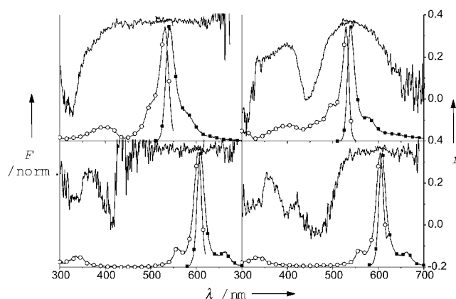
Figure 5. Fluorescence excitation (○) and emission (●) spectra of 3a (upper left), 3b (upper right), 4a (lower left), and 4b (lower right) in propylene glycol at 223 K. The corresponding anisotropies are included.
