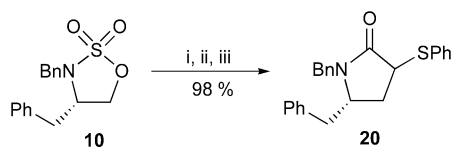
Scheme 4 Reagents and conditions: (i), 9b , NaH, DMF, r.t.; (ii), 5M HCl then NaHCO 3 ; (iii), PhMe, reflux. See Table 1 for other substrates studied.
