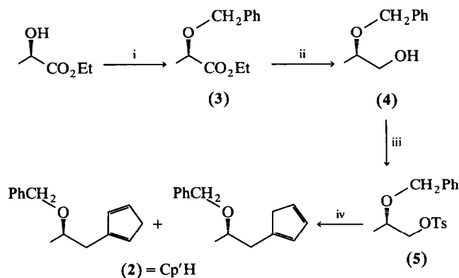
Scheme 1. (i) Benzyl trichloroacetimidate, \text{CF}_3\text{SO}_3\text{H} cat, \text{C}_6\text{H}_{12}/\text{CH}_2\text{Cl}_2 (2:1), 70% yield, 97% ee; (ii) \text{LiAlH}_4 , \text{Et}_2\text{O} , 0°C to room temperature, 84% yield, 93% ee; (iii) TsCl, pyridine, 0°C, 91% yield; (iv) \text{NaCp} , THF, 84% yield.
