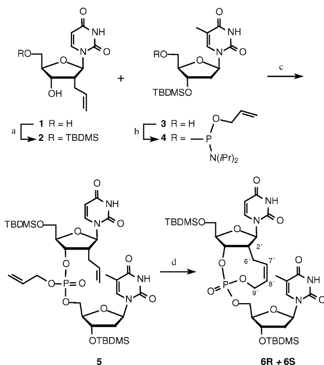
Scheme 1 Reagents and conditions: a) TBDMSCl, AgNO 3 , pyridine, 85%; b) CH 2 =CHCH 2 OP(N i Pr) 2 , 1 H -tetrazole, CH 3 CN, 66%; c) i) 1 H -tetrazole, CH 3 CN, ii) t BuOOH, toluene, CH 3 CN, 85%; d) Grubbs 2 nd gen. catalyst, § CH 2 Cl 2 , 40% 6R , 20% 6S , 16% mixture. TBDMS = t -butyldimethylsilyl.
