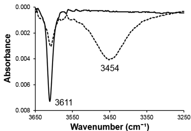
Figure 1. Representative IR spectrum of phenol in \text{CCl}_4 (solid line) and in 1% \text{CD}_3\text{CN}/\text{CCl}_4 (dotted line).
