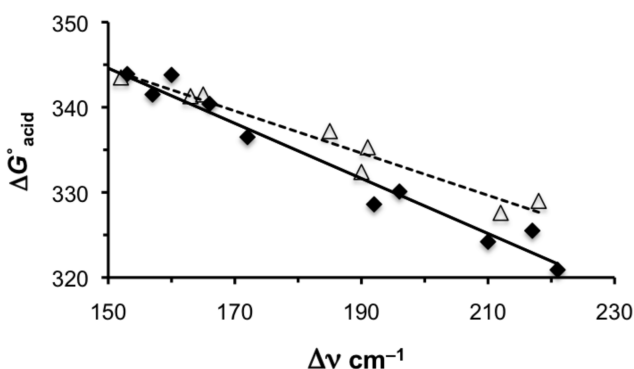
Figure 3. Gas phase acidities ( \text{kcal mol}^{-1} ) vs O–H frequency shifts for m- (triangles) and p-substituted (diamonds) phenols. Linear least-squares analyses give y(\text{pK}_a) = -0.241(\Delta\nu) + 380.3 , r^2 = 0.950 (meta) [dotted line] and y(\text{pK}_a) = -0.324(\Delta\nu) + 393.2 , r^2 = 0.970 (para) [solid line].
