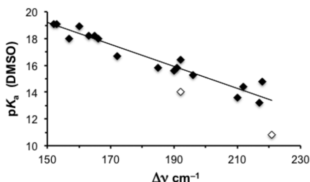
Figure 2. DMSO \text{pK}_a values vs m- and p-substituted phenol O–H frequency shifts in \text{CCl}_4 upon addition of \text{CD}_3\text{CN} . A linear least-squares fit of the data affords y(\text{pK}_a) = -0.0822(\Delta\nu) + 31.6 , r^2 = 0.936 , where the open diamonds are for the p\text{-NO}_2 and p\text{-COCH}_3 derivatives, which were excluded from the analysis.
