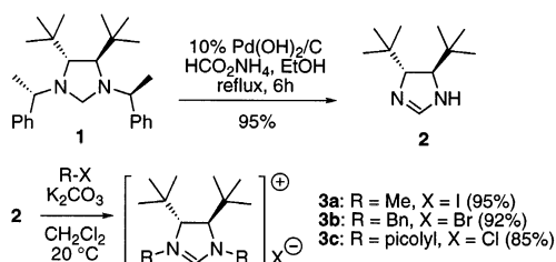
Scheme 1. Preparation of imidazolinium salts from ( R,R )-4,5-di- tert -butylimidazolidine ( 2 ).
