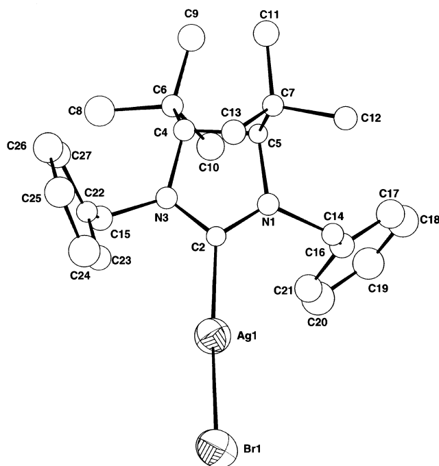
Fig. 3. ORTEP view of silver(I) diaminocarbene 5b .
