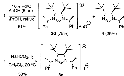
Scheme 2. Preparation of imidazolinium salts by oxidation of aминаl 1 .
