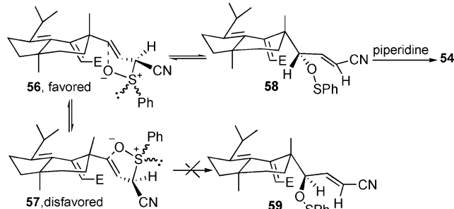
Scheme 11. Mechanistic Rationale for the Hydroxylative Knoevenagel Reaction to Form 54
