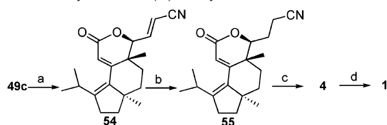
Scheme 10. Synthesis of (+)-Alloocyathin B 2 a
