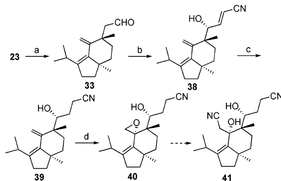
Scheme 7. Synthesis of Epoxide 40 a
