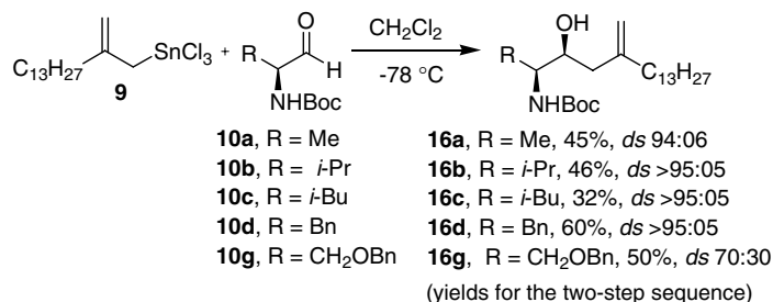
Scheme 5. Coupling with allyltrichlorostannane 9 .
