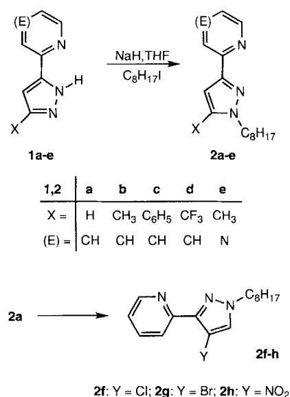
Scheme 3. Synthesis of the N -octylated 2-(3-pyrazolyl)pyridines 2a – h .
