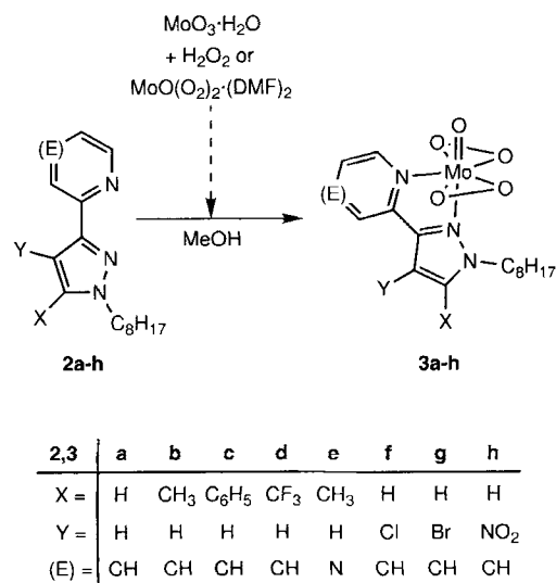
Scheme 4. Synthesis of the molybdenum peroxo complexes 3a–h .
