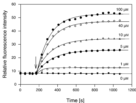
Fig. 6. Time evolution of NO release from MAHMA NONOate as monitored by trapping with FNOCT 14 at pH 7.4. [ 14 ] = 10 \mu\text{M} , [phosphate buffer] = 50 mM, [Trolox] = 100 \mu\text{M} , [dtpa] = 100 \mu\text{M} ; \lambda_{\text{exc}} 320 nm, \lambda_{\text{em}} 380 nm; T 37°. The arrow marks the point of addition of MAHMA NONOate; numbers indicate the initial concentration of MAHMA NONOate. Solid lines are least-squares fits to a first-order rate law.
