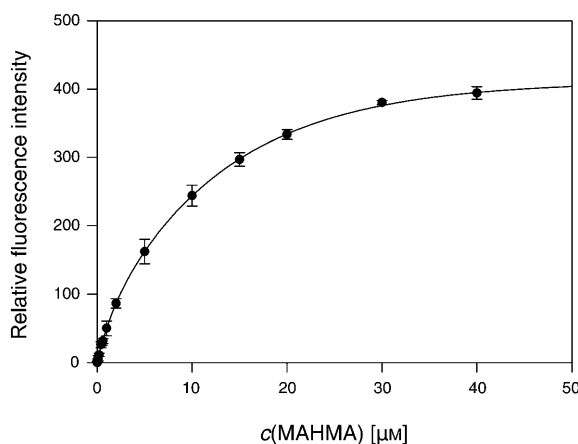
Fig. 7. Efficiency of NO trapping by FNOCT 14 at pH 7.4 as a function of the concentration of the NO donor MAHMA NONOate. [ 14 ] = 10 \mu\text{M} , [phosphate buffer] = 50 mM, [Trolox] = 100 \mu\text{M} , [dtpa] = 100 \mu\text{M} ; \lambda_{\text{exc}} 320 nm, \lambda_{\text{em}} 380 nm; T 37°.
