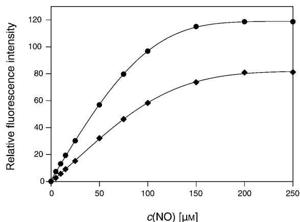
Fig. 5. NO Trapping by FNOCT 14 as a function of added NO at pH 7.35. [ 14 ] = 50 \mu\text{M} , [phosphate buffer] = 50 mM, [ascorbic acid] = 100 \mu\text{M} ; ● oxygen-free buffer, ◆ air-saturated buffer.
