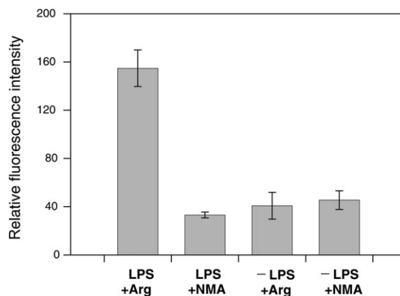
Fig. 9. Trapping of NO produced by rat alveolar macrophages. LPS + Arg : Cells activated with LPS (0.5 \mu\text{g}/\text{ml} , 18 h) in the presence of L-arginine (0.5 mM); LPS + NMA : Cells activated with LPS (0.5 \mu\text{g}/\text{ml} , 18 hrs) in the presence of the NO-synthase inhibitor NMA (0.1 mM); -LPS + Arg : Cells incubated with L-arginine (0.5 mM), no pretreatment with LPS; -LPS + NMA : Cells incubated with NMA (0.1 mM), no pretreatment with LPS. All experiments were performed in Krebs–Henseleit buffer, [\text{D-glucose}] = 10 \text{ mM} , [\text{dtpa}] = 100 \mu\text{M} , [\text{Trolox}] = 100 \mu\text{M} , [14] = 10 \mu\text{M} ; incubation time 1 h, T 37^\circ . Fluorescence intensity ( \lambda_{\text{exc}} 320 , \lambda_{\text{em}} 380 \text{ nm} ) shown is the sum of the fluorescence from the supernatant and cell-associated fluorescence as determined in the cell lysates (corrected for volume, background, and cell density).
