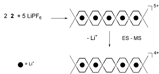
Scheme 13. Formation of complexes [(2)_2\cdot 5\text{Li}]^{5+}\cdot(5\text{PF}_6)^{5-} and [(2)_2\cdot 4\text{Li}]^{4+}\cdot(4\text{PF}_6)^{4-} .
