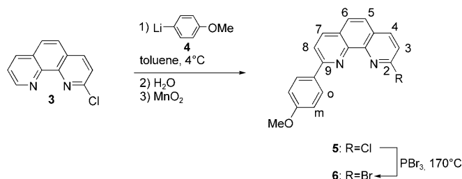
Scheme 3. Synthesis of 2-bromo-9-( p -anisyl)phenanthroline ( 6 ).
