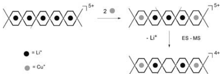
Scheme 14. Heteronuclear complexes [(2)_2\cdot 3\text{Li}\cdot 2\text{Cu}]^{5+}\cdot(5\text{PF}_6)^{5-} and [(2)_2\cdot 2\text{Li}\cdot 2\text{Cu}]^{4+}\cdot(4\text{PF}_6)^{4-} .
