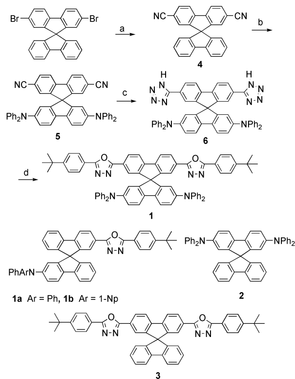
Scheme 1 Reagents and condition: a, CuCN, DMF, reflux; b, i, Br 2 , AlCl 3 , CH 2 Cl 2 , reflux; ii, Ph 2 NH, Pd(OAc) 2 , P(t-Bu) 3 , NaOtBu, PhCH 3 , reflux; c, NaN 3 , NH 4 Cl, DMF, reflux; d, 4- t -BuPhCOCl, pyridine, reflux.
