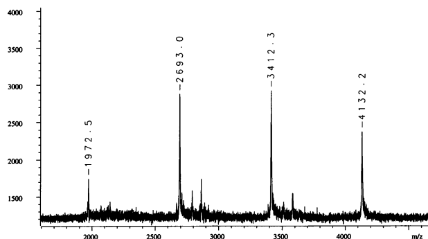
Figure 4. MALDI-TOF mass spectrum of nanotruck 1a . Peaks for one-, two-, three-, and four-wheel nanotrucks ( m/z 1972.5, 2693.0, 3412.3, and 4132.2, respectively) are observed (negative ion mode, dithranol matrix).
