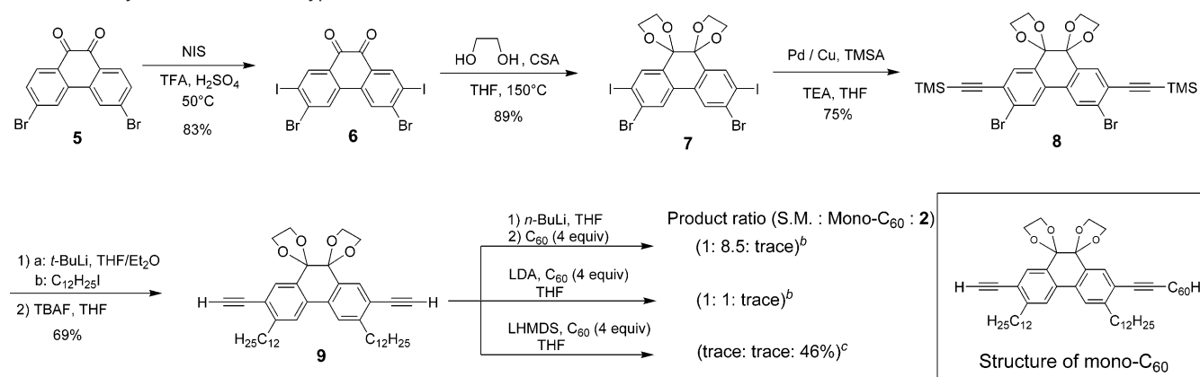
Scheme 1. Synthesis of the Prototype: Half-Truck a
