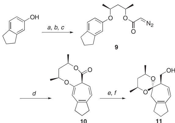
Scheme 3. Reagents and conditions. a: (2 R ,4 R )-2,4-pentane-diol/diisopropyl azodicarboxylate/PPh 3 (74.3%), b: diketene/triethylamine (91.2%), c: TsN 3 /triethylamine, then 1 M NaOH aq (87.3%), d: Rh 2 (OAc) 4 (82.8%), e: LiAlH 4 /–78 °C (quant.), f: TsOH·Py/THF/rt (70.6%).
