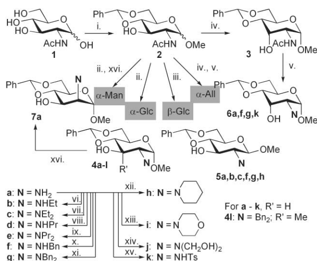
Scheme 1 Reagents and conditions: (i) MeOH, AcCl, 100% then PhCH(OMe) 2 , pTsOH, DMF, 70 °C, 69%; (ii) (iii) N 2 H 4 , 130 °C, 88%, or 4 M KOH, EtOH, -70–85%; (iv) DMSO, (CF 3 CO) 2 O, Et 3 N, DCM, -78 °C, 75% then L-selectride, THF, -78 °C, 75 then 60% 2 → 3 , 52 then 74% 4b → 6b , 80 then 60% 4c → 6c ; (v) 4 M KOH, EtOH, Δ, 49%; (vi) 1.1 eq. EtI, K 2 CO 3 , MeCN, 60 °C, 56% for 4a → 4b , 42% for 5a → 5b ; (vii) 2.1 eq. EtI, K 2 CO 3 , MeCN, 60 °C, 84% for 4a → 4c , 80% for 5a → 5c ; (viii) 1.1 eq. PrI, K 2 CO 3 , MeCN, reflux, 63% for 4a → 4d ; (ix) 3 eq. PrI, K 2 CO 3 , MeCN, reflux, 72% for 4a → 4e , 42% for 5a → 5b ; (x) 2 eq. TMSCl, DIPEA, DCM then BnBr, Bu 4 NI then Bu 4 NF, THF, 56% for 4b , 61% for 5b ; (xi) 1 eq. TMSCl, DIPEA, DCM then BnBr, Bu 4 NI then Bu 4 NF, THF, 68% for 4c , 75% for 5c ; (xii) 1.1 eq. I(CH 2 ) 5 I, K 2 CO 3 , MeCN, 60 °C, 85% for 4a → 4h , 90% for 5a → 5h ; (xiii) 1.1 eq. I(CH 2 ) 2 O(CH 2 ) 2 I, K 2 CO 3 , MeCN, 70 °C, 91% for 4a → 4i , 75% for 5a → 5i ; (xiv) 3 eq. I(CH 2 ) 2 OH, K 2 CO 3 , MeCN, reflux, 39% for 4a → 4j ; (xv) TsCl, Et 3 N, DCM, 75% for 4d , 60% for 6d ; (xvi) H 2 O 2 , Na 2 WO 4 , MeOH–H 2 O, 46% then LiAlH 4 , THF, 0→50 °C, 28% for 7a .
