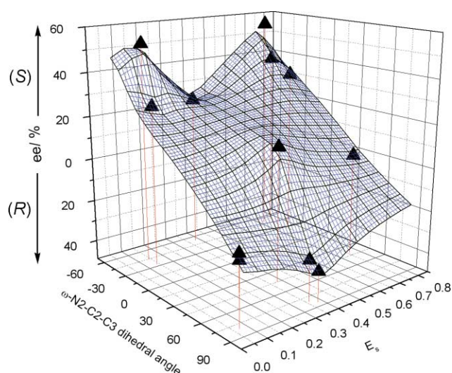
Fig. 3 Enantioselectivity surface graph for the \omega -N2–C2–C3 dihedral angle vs. N -steric bulk as judged by Taft's steric parameter, E_s . N -alkyl and N -benzyl substituted ligands and corresponding dihedral angles taken from X-ray structures and molecular modeling calculations are shown. 4b \omega -N2–C2–C3 dihedral angle = 80.9°, O1–C1–C2–N2 dihedral angle = 53.4°, E_s = 0.07; 4c –44.5°, 60.3°, 0.14; 4d 80.9°, 53.4°, 0.36; 4e –49.9°, 59.4°, 0.72; 4f 85.4°, 51.9°, 0.38; 4g –51.1°, 61.3°, 0.76; 5b 80.8°, –66.5°, 0.07; 5c –33.3°, –59.0°, 0.14; 5f 45.0°, –56.9°, 0.38; 5g –28.6°, –58.9°, 0.76; 6f –52.3°, 42.6°, 0.38; 6g 41.1°, 57.6°, 0.76. A moderate increase in selectivity with the steric parameter is observed over this range. Far more striking is the relationship between calculated \omega -N2–C2–C3 dihedral angle and selectivity. ( R ) stereoselectivity is favoured by dihedral angles in the range 80–90°, whilst the more common ( S ) stereoselectivity is found when the dihedral angle is negative ( i.e. the lone pair is above the plane of the sugar ring). When the dihedral angle is in the range 40–45° very low enantioselectivity is observed.
