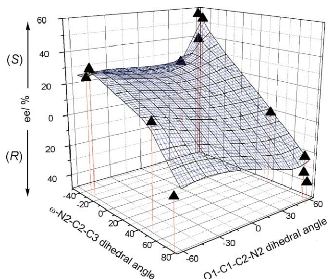
Fig. 4 Enantioselectivity surface graph for the \omega -N2–C2–C3 dihedral angle vs. the O1–C1–C2–N2 dihedral angle. Values used are given in the caption to Fig. 3. The enhanced selectivity and greater variability at an O1–C1–C2–N2 dihedral angle of 60° (for both ( S ) and ( R ) enantiomers) is apparent. The dependency of the sense of induction on \omega -N2–C2–C3 dihedral angle is once again clear also.
