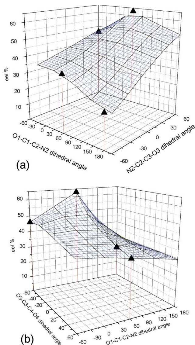
Fig. 2 Enantioselectivity surface graphs for the primary amine ligands, 4a , 5a , 6a and 7a . (a) O1–C1–C2–N2 dihedral angle vs. N2–C2–C3–O3 dihedral angle. (b) O1–C1–C2–N2 dihedral angle vs. O3–C3–C4–O4 dihedral angle. These plots indicate the effect of changing the configuration at the C1, C2 and C3 positions; the importance of the N2–C2–C3–O3 dihedral angle is apparent since the gradient of the surface parallel to the N2–C2–C3–O3-axis is greater than that parallel to the O1–C1–C2–N2-axis. The \alpha -gluco stereochemistry is thus confirmed as the optimum ligand configuration within these 4 ligand diastereomers.
