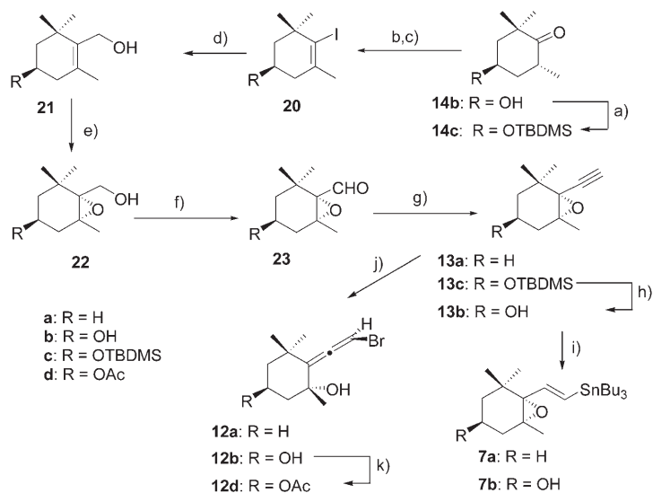
Scheme 5. a) TBDMSCl, imidazole, DMF, 25 °C (83 %); b) H 2 NNH 2 ·H 2 O, Et 3 N, EtOH, reflux; c) I 2 , DBN, EtO 2 (2 steps, 80 %); d) t BuLi, (CH 2 O) n , THF, –78 °C, 15 h (71 %); e) D-(–)-DET, Ti(O i Pr) 4 , TBHP, CH 2 Cl 2 , –20 °C (98 % for 22a , 98 % for 22c ); f) (COCl) 2 , DMSO, Et 3 N, CH 2 Cl 2 , –60 to 25 °C (89 % for 23a , 91 % for 23c ); g) LDA, TMSCHN 2 , THF, –78 to 25 °C (84 % for 13a , 92 % for 13c ); h) TBAF, THF, 25 °C, 2 h (85 % for 13b ); i) [PdCl 2 (PPh 3 ) 2 ], Bu 3 SnH, THF, 25 °C (70 % for 7a , 68 % for 7b ); j) CuBr, NH 4 Br, HBr, Et 2 O, –10 °C (86 % for 12a , 85 % for 12b ); k) Ac 2 O, py, 25 °C, 16 h (85 %). TBDMS = tert -butyldimethylsilyl; DBN = 1,5-diazabicyclo[4.3.0]non-5-ene; DET = diethyl D-tartrate; TBHP = tert -butyl hydroperoxide; LDA = lithium diisopropylamide; TBAF = tetrabutylammonium fluoride.
