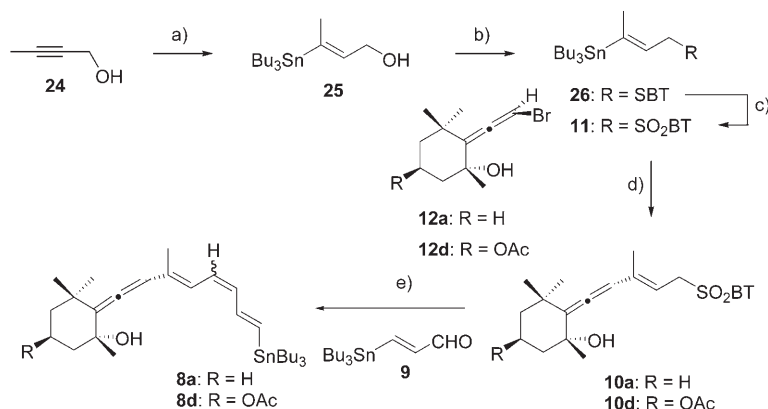
Scheme 6. a) (\text{Bu}_3\text{Sn})_2 , n\text{-BuLi} , \text{CuCN} , \text{MeOH} , \text{THF} , -10^\circ\text{C} (89%); b) BTSH, \text{PPh}_3 , DIAD, \text{THF} , 25^\circ\text{C} (98%); c) 35% \text{H}_2\text{O}_2 , (\text{NH}_4)_6\text{Mo}_7\text{O}_{24}\cdot 4\text{H}_2\text{O} , \text{EtOH} , 25^\circ\text{C} (56%); d) (aR)- 12 , [\text{Pd}(\text{PhCN})_2\text{Cl}_2] , (i\text{Pr})_3\text{NEt} , \text{DMF/THF} , 40^\circ\text{C} (69% for 10a , 64% for 10d ); e) 10 , \text{NaHMDS} , \text{THF} , -78^\circ\text{C} , then 9 (79% for 8a , 70% for 8d ). BTSH = 2-mercaptobenzothiazole; HMDS = hexamethyldisilazane.
