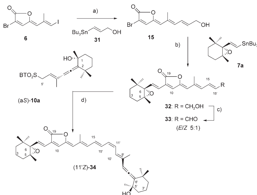
Scheme 9. a) [\text{Pd}_2(\text{dba})_3]\cdot\text{CHCl}_3 , [\text{AsPh}_3] , \text{Bu}_4\text{N}^+\text{Ph}_2\text{PO}_2^- , THF, 25 °C, 4.5 h (68 %); b) [\text{Pd}_2(\text{dba})_3]\cdot\text{CHCl}_3 , [\text{AsPh}_3] , \text{Bu}_4\text{N}^+\text{Ph}_2\text{PO}_2^- , THF, 50–55 °C, 20 h (45 %); c) TPAP, NMO, \text{CH}_2\text{Cl}_2 , 25 °C (36 %); d) NaHMDS, THF, -78^\circ\text{C} \rightarrow 0^\circ\text{C} (63 %). TPAP = tetra- n -propylammonium perruthenate; NMO = N -methylmorpholine N -oxide.
