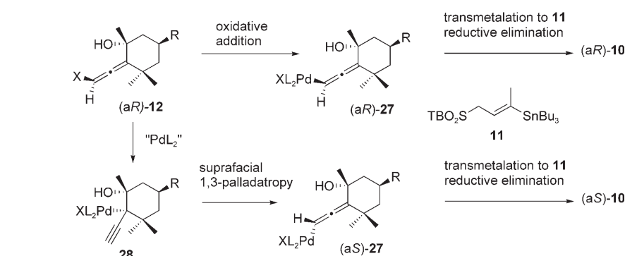
Scheme 7. Alternative pathways for the reaction of haloallenes 12 and stannane 11 catalyzed by palladium complexes.
