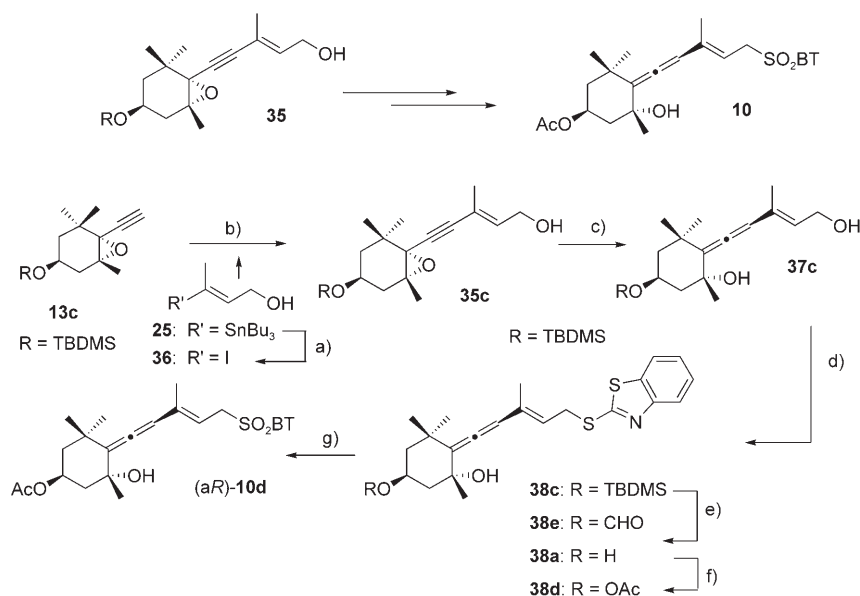
Scheme 10. a) \text{I}_2 , \text{CH}_2\text{Cl}_2 , 25 °C (98 %); b) [\text{Pd}(\text{PPh}_3)_4] , CuI, (i\text{Pr})_2\text{NH} , 25 °C (78 %); c) DIBAL, \text{CH}_2\text{Cl}_2 , 0 °C (99 %); d) BTSH, DIAD, \text{PPh}_3 , THF, 0 °C (100 %); e) \text{HCO}_2\text{H} , THF, \text{H}_2\text{O} , 25 °C; f) \text{Ac}_2\text{O} , Py, 25 °C (99 % combined yield); g) 35 % \text{H}_2\text{O}_2 , (\text{NH}_4)_6\text{Mo}_7\text{O}_{24}\cdot 4\text{H}_2\text{O} , EtOH, -10^\circ\text{C} (93 %). DIBAL = diisobutylaluminium hydride.
