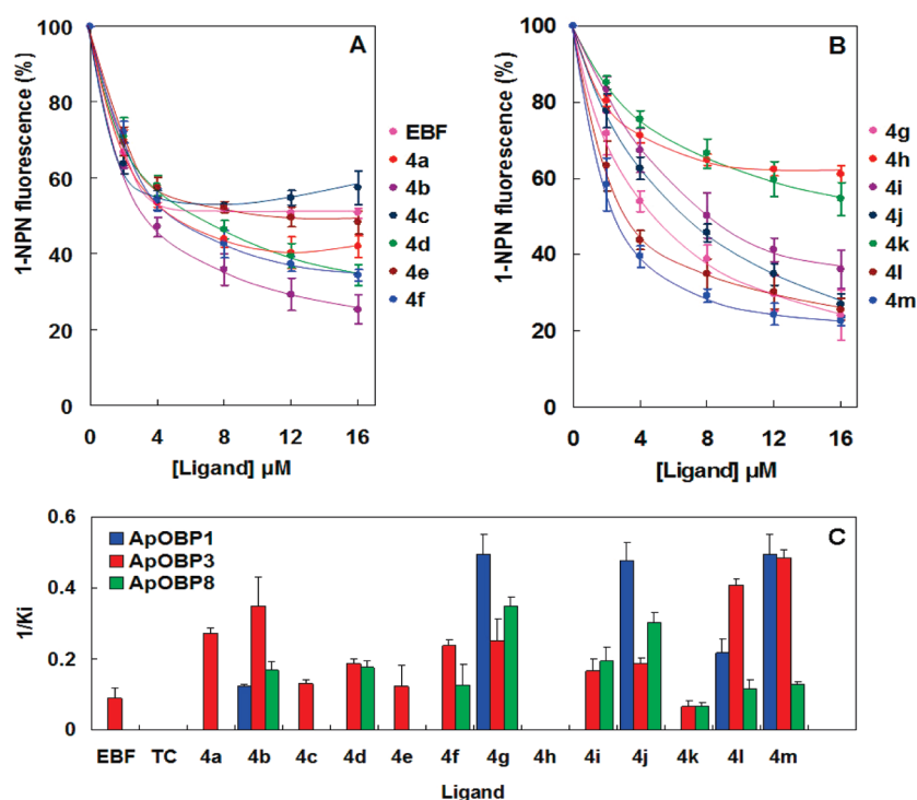
Figure 2. Competitive binding of the compounds prepared to OBPs of A. pisum . (A, B) Displacement curves of the fluorescent probe 1-NPN from the complex with OBPs by each synthetic compound. A solution of 2 μM protein and 2 μM 1-NPN in Tris was titrated with aliquots of 1 μM solution of the ligand up to the final concentration of 16 μM. Fluorescence intensities are reported as percent of the values in the absence of competitor. Parallel experiments were also performed with OBPs 1 and 8 (data not shown). (C) Comparison of the affinity of each ligand to the three OBPs used. Reciprocal of dissociation constants (divided by 10 6 ) are reported, as calculated from the concentration values of each ligand halving the initial fluorescence value. EBF: ( E )-β-farnesene. TC: thiacloprid. The structures of all the ligands are reported in Figure 1.
