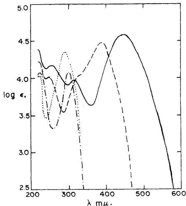
Fig. 1.—Ultraviolet absorption data: ..... chalcone (in hexane); ——— dehydroacetic acid; ..... 3-(3',4'-dimethoxycinnamoyl)-4-hydroxy-6-methyl-2-pyrone; ——— 3-( p -dimethylaminophenyl)-4-hydroxy-6-methyl-2-pyrone.
