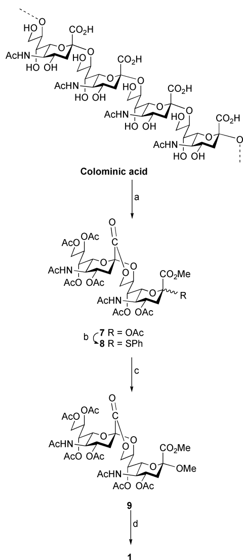
Scheme 2 Reagents and conditions: a. 1) \text{H}_2\text{O} , pH = 3.8, 70^\circ\text{C} ; 2) \text{MeOH}/\text{Dowex} (\text{H}^+) , then \text{HCl}/\text{MeOH} ; 3) \text{Ac}_2\text{O}/\text{Py} ; b. \text{PhSH} , \text{BF}_3 \cdot \text{Et}_2\text{O}/\text{CH}_2\text{Cl}_2 ; c. \text{MeOH} , NIS, \text{TfOH}/\text{CH}_3\text{CN} , -35^\circ\text{C} ; d. \text{NaOMe}/\text{MeOH} ; then \text{H}_2\text{O} .
