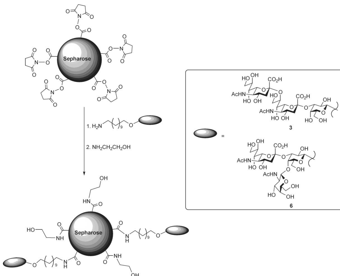
Scheme 9
