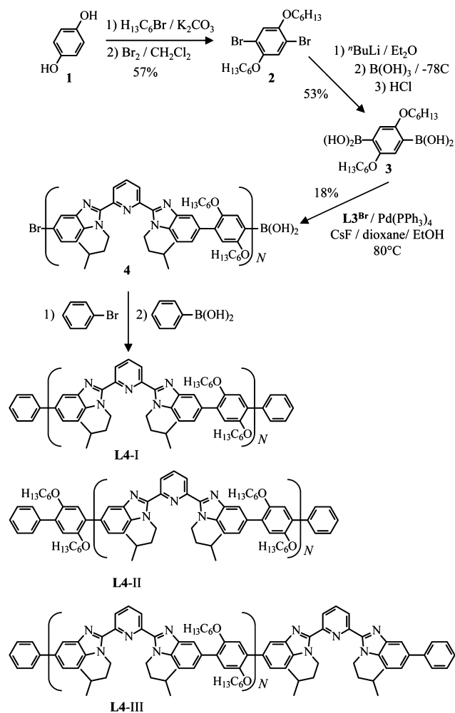
Scheme 3. Synthesis of Polymer L4 Highlighting the Three Planned Possible Termini
