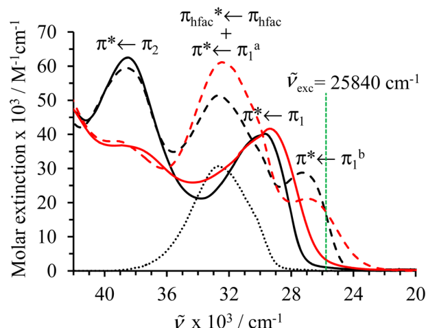
Figure 8. Electronic absorption spectra per tridentate binding site recorded for L3 Ph (black full trace), L4 (red full trace), [Eu(hfac)_3(L3^{Ph})] (black dashed trace), [Eu(hfac)_3]_m(L4) (red dashed trace), and [Eu(hfac)_3(dig)] (black dotted trace) in CH_2Cl_2 + 10^{-4} M diglyme at 293 K. The absorption spectra were recorded for [Eu]_{tot} = 7 \times 10^{-5} M and corrected for partial dissociation in solution (see Appendix 5). The vertical dotted green trace indicates the excitation energy used for recording the emission spectra of the complexes.
