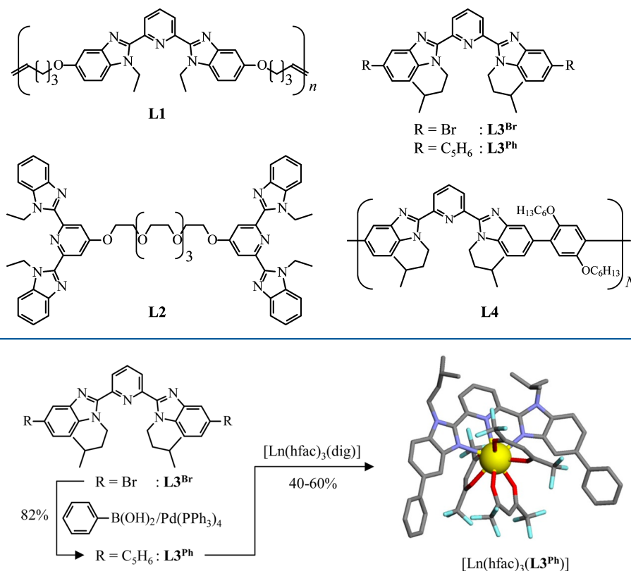
Figure 2. Synthesis of ligand L3 Ph and of its mononuclear complexes [Ln(hfac) 3 (L3 Ph )]. A perspective view of the X-ray diffraction molecular structure of [La(hfac) 3 (L3 Ph )] is shown on the right.
