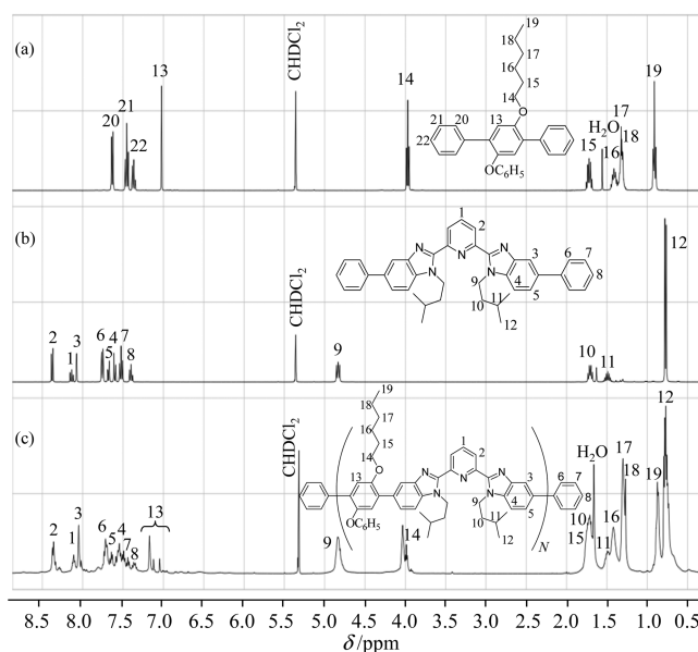
Figure 5. ^1\text{H} NMR spectra with assignments and numbering schemes for (a) para-disubstituted 1,4-dihexyloxy-benzene bridge, (b) central tridentate binding unit in \text{L}^3\text{Ph} , and (c) polymer L4 .
