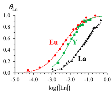
Figure 7. Occupancy factors deduced from the ^1\text{H} NMR titrations of L4 (3 mM) with [\text{Ln}(\text{hfac})_3] ( \blacktriangle = La (black), \bullet = Eu (red), and \blacksquare = Y (green)) in \text{CD}_2\text{Cl}_2 + 0.14 M dig at 293 K. The dotted lines correspond to the theoretical binding isotherms fitted with eq 11 for the mixture of oligomers N = 18 (0.16), N = 11 (0.18), N = 9 (0.19), N = 6 (0.25), N = 5 (0.15), N = 4 (0.06), and N = 3 (0.01).
