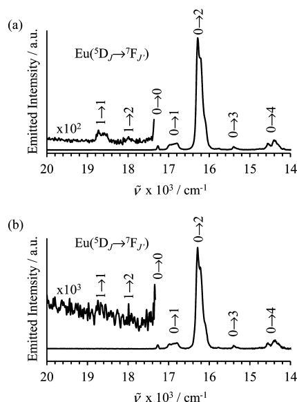
Figure 9. Emission spectra recorded for (a) [Eu(hfac)_3(L3^{Ph})] ( 10^{-5} M, \theta_{Eu} = 0.98 ) and (b) [Eu(hfac)_3]_m(L4) ( 6 \times 10^{-6} M, \theta_{Eu} = 0.85 ) in CH_2Cl_2 + 10^{-4} M diglyme at 293 K upon excitation at \tilde{\nu}_{exc} = 25\,840 cm^{-1} .
