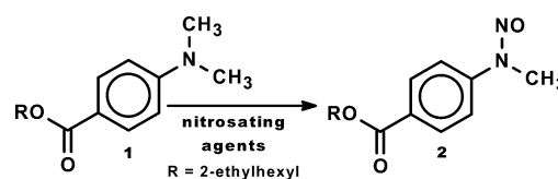
Scheme 1 Nitrosation of Padimate-O.
