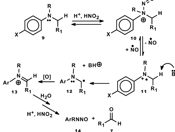
Scheme 3 Mechanism B: deprotonation of radical cation.
