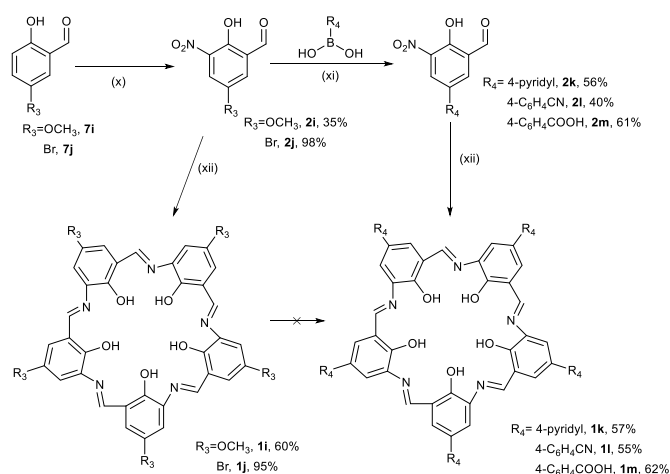
Scheme 3 Syntheses of campestarenes ( 1i-1m ): (x) \text{HNO}_3 , \text{AcOH} , 2 h; (xi) \text{Na}_2\text{CO}_3 , \text{Pd}(\text{PPh}_3)_4 , \text{DMF}/\text{H}_2\text{O} , 105^\circ\text{C} , 6 h, then \text{HCl} ; (xii) \text{Na}_2\text{S}_2\text{O}_4 , \text{EtOH}/\text{H}_2\text{O} , reflux, 2 h.
