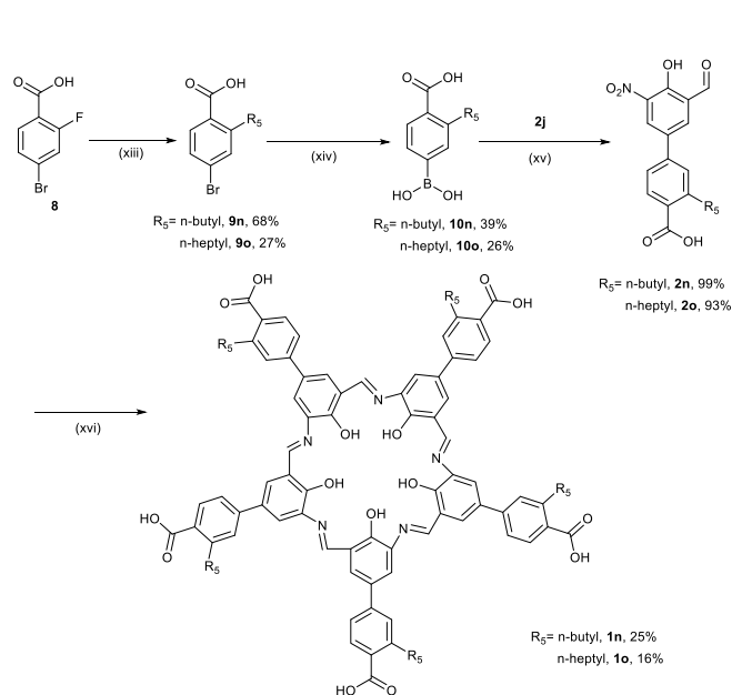
Scheme 4 Syntheses of campestarenes ( 1n and 1o ): (xiii) \text{R}_5\text{MgBr} , \text{THF} , \text{N}_2 , 17 h, then \text{HCl} ; (xiv) n\text{-BuLi} , \text{B}(\text{O}-i\text{-Pr})_3 , \text{THF} , -78^\circ\text{C} , 3 h, then \text{HCl} ; (xv) \text{Na}_2\text{CO}_3 , \text{Pd}(\text{PPh}_3)_4 , \text{DMF}/\text{H}_2\text{O} , 105^\circ\text{C} , 6 h; (xvi) \text{Na}_2\text{S}_2\text{O}_4 , \text{EtOH}/\text{H}_2\text{O} , reflux, 2 h.
