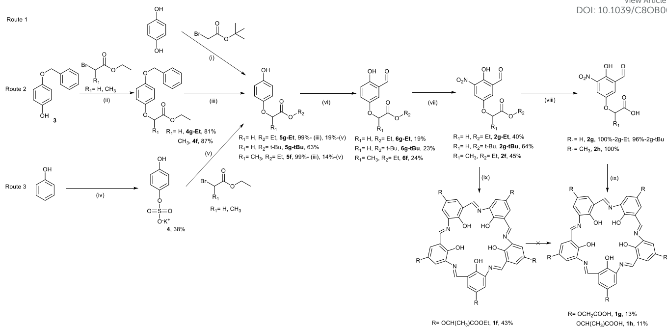
Scheme 2 Syntheses of ester/carboxylic acid campesterenes ( 1f-1h ): (i) NaOH, dioxane/H 2 O, 3 h, then HCl; (ii) K 2 CO 3 , acetone, reflux, 3 h, then HCl; (iii) Pd/C, H 2 , EtOH, 12 h; (iv) K 2 S 2 O 8 , NaOH, H 2 O, 24 h, then HCl; (v) K 2 CO 3 , EtOH, reflux 6 h, then AcOH, reflux, 2 h; (vi) Et 3 N, MgCl 2 , CH 2 O, MeCN, reflux, 24 h, then HCl; (vii) HNO 3 , AcOH, 2 h; (viii) R 2 = Et, NaOH, MeOH/H 2 O, 12 h, then HCl or R 2 = t-Bu, TFA/DCM, 12 h; (ix) Na 2 S 2 O 4 , EtOH/H 2 O, reflux, 2 h.
