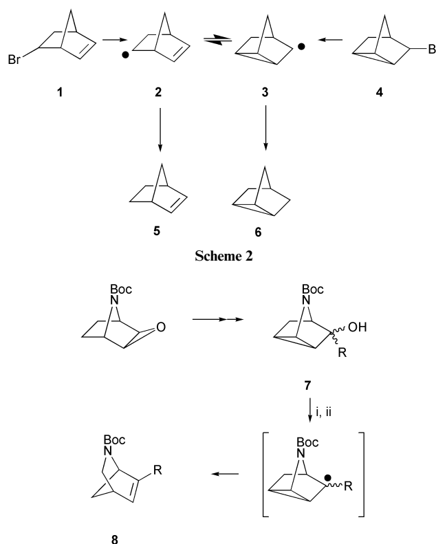
Scheme 3 Reagents and conditions: i, ClCOCOMe, DMAP, MeCN, 25 °C, 30 min; ii, Bu 3 SnH, AIBN, toluene, 100 °C, 45 min.
