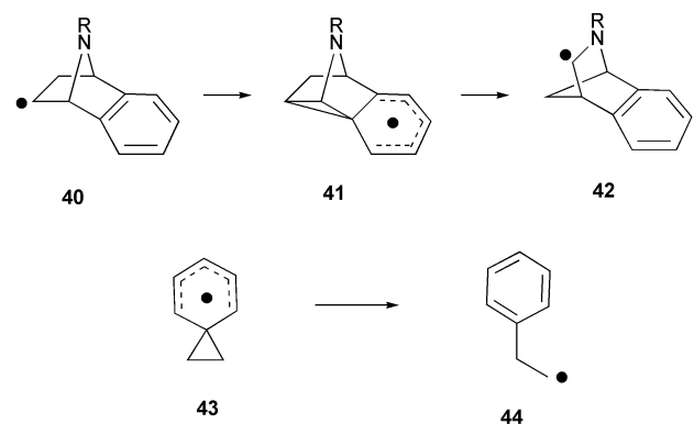
Scheme 16
