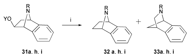
Scheme 15 Reagents and conditions: i, TTMSS, AIBN, toluene, reflux, 2 h.
