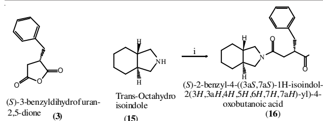
Scheme-VII: Reagents and conditions: (i) Toluene, 40-45 °C
