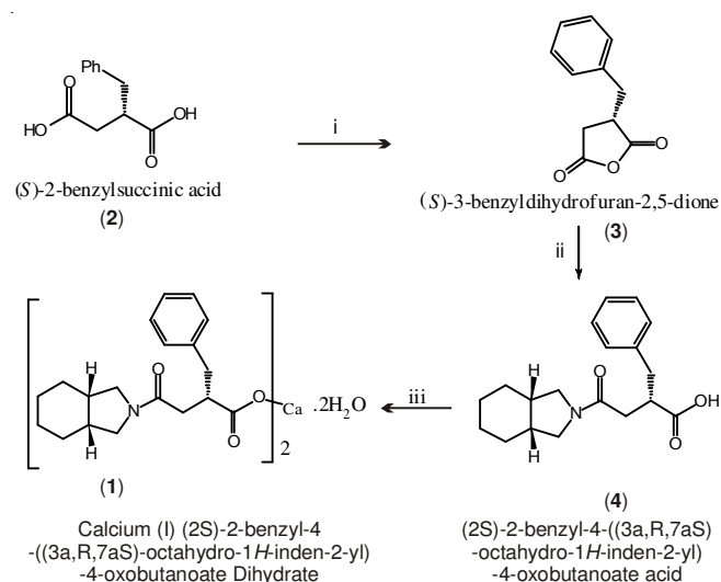
Scheme-I: Reagents and conditions: (i) Dichloromethane, acetic anhydride, 40-45 °C; (ii) cis -Octahydroisoindole, toluene, 40-45 °C; (iii) NaOH, \text{H}_2\text{O} , calcium chloride, ethanol
