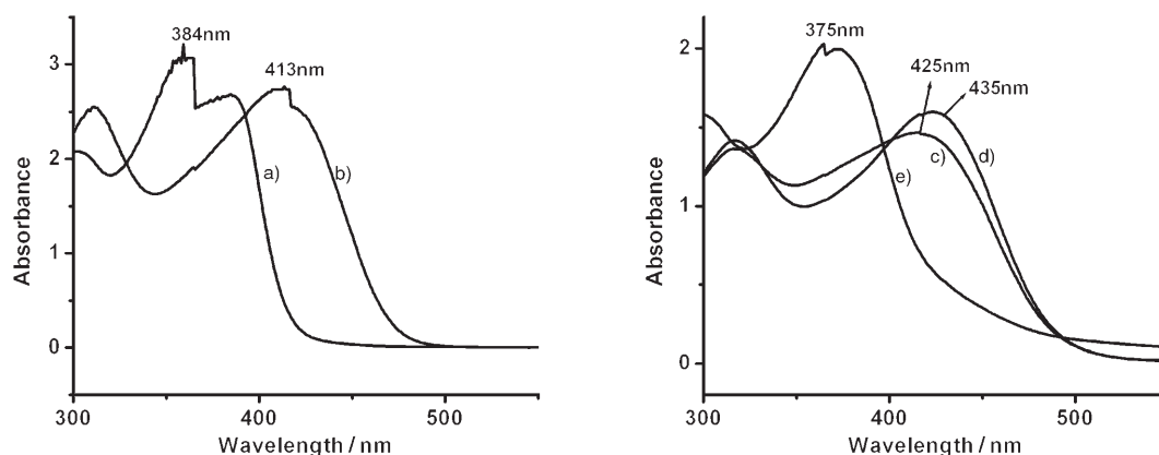
Figure 7. Absorption spectra in neutral pH for polymer P1 (a) and P4 (c), in the presence of \text{H}^+ for P1 (b) and P4 (d), in the presence of \text{OH}^- for polymer P4 (e) in chloroform at room temperature. Concentrations of P1 and P4 were 3.06 \times 10^{-5} \text{ M} and 3.52 \times 10^{-5} \text{ M} , respectively. Note the redshift in \lambda_{\text{max}} caused by protonation and the blueshift caused by deprotonation. Absorbance has arbitrary units.
