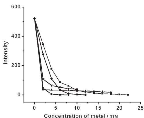
Figure 11. Titration traces of metal ions ( Cu ■, Fe ●, Ag ▲, Ni ▼, Pd ◆) added to polymer P4 in THF (concentration of P4 is 3.52 \times 10^{-5} M). Intensity has arbitrary units.
