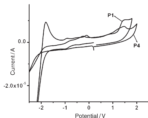
Figure 3. Cyclic voltammogram of a thin film of polymers P1 and P4 recorded with a glassy carbon electrode under a nitrogen atmosphere. CV traces of the other polymers are given in the Supporting Information.
