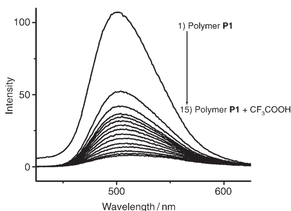
Figure 8. Changes in the emission spectra of P1 in chloroform at different concentrations (in mM) of \text{CF}_3\text{COOH} : 1) 0, 2) 4, 3) 8, 4) 12, 5) 16, 6) 20, 7) 24, 8) 28, 9) 40, 10) 60, 11) 80, 12) 120, 13) 240, 14) 320, and 15) 400 mM in methanol. The concentration of P1 was 3.06 \times 10^{-5} \text{ M} . Data of other polymers are given in the Supporting Information. Intensity has arbitrary units.
