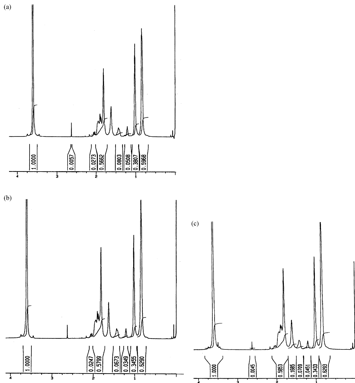
Fig. 6. (a) ^1\text{H} -NMR plot for PMMA catalyzed by (\text{CH}_2=\text{CHCH}_2\text{CH}_2\text{C}_5\text{H}_4)_2\text{Sm}-\text{Cl}\cdot 2\text{THF} , run B18. (b) ^1\text{H} -NMR plot for PMMA catalyzed by (\text{CH}_2=\text{CHCH}_2\text{CH}_2\text{C}_5\text{H}_4)_2\text{Sm}-\text{Cl}\cdot 2\text{THF} , run B21. (c) ^1\text{H} -NMR plot for PMMA catalyzed by (\text{CH}_2=\text{CHCH}_2\text{CH}_2\text{C}_5\text{H}_4)_2\text{Sm}-\text{Cl}\cdot 2\text{THF} , run B4.
