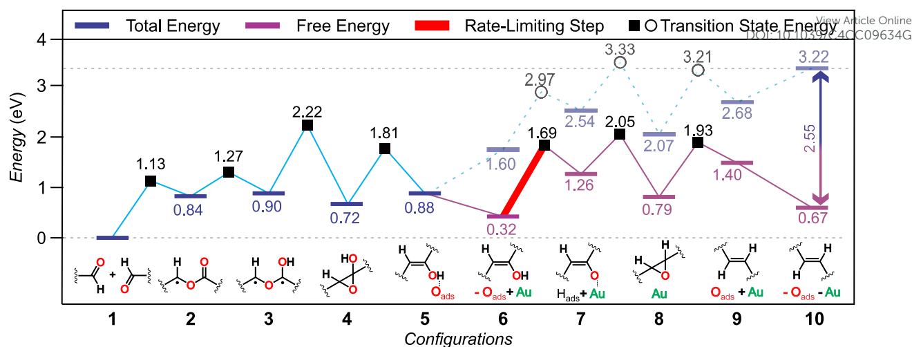
Fig. 4 Energetics of the proposed reaction mechanism. Purple lines indicate free energy estimates after oxygen desorption at the experimental conditions. The rate limiting step appears highlighted in red.
