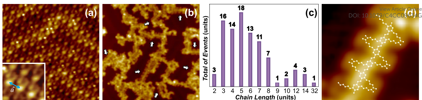
Fig. 2 Deposition and on-surface reaction of DTA monomers on Au(111). a) STM image ( 12 \times 12 \text{ nm}^2 ; U = -1.50 \text{ V} ; I = 400 \text{ pA} ) after the deposition onto the surface kept at room temperature. The inset shows the intermolecular distance between adjacent monomers along the aldehyde moiety direction. b) STM image ( 30 \times 30 \text{ nm}^2 ; U = -0.65 \text{ V} ; I = 7 \text{ pA} ) after the deposition onto the surface kept at 250^\circ\text{C} . The targeted coupling reaction is achieved, producing p -PPV oligomers (white arrows) on the surface. c) Oligomers 2 chain length distribution. d) High resolution STM image ( 5.7 \times 8.5 \text{ nm}^2 ; U = 0.65 \text{ V} ; I = 7 \text{ pA} ) of the p -PPV products 2 . The inset schematically represents the chemical structure of the reacted specie.
