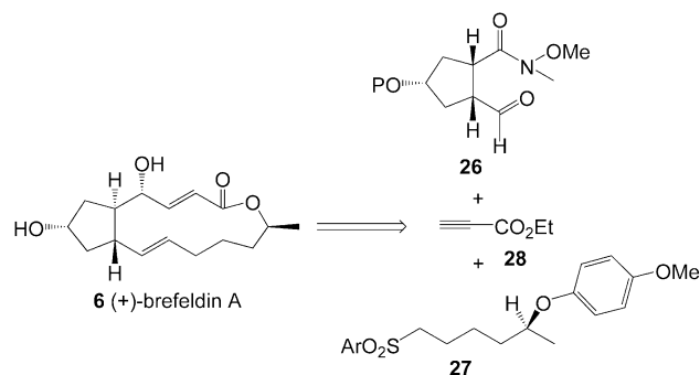
Scheme 3. Retrosynthetic analysis of (+)-brefeldin A ( 6 ).
