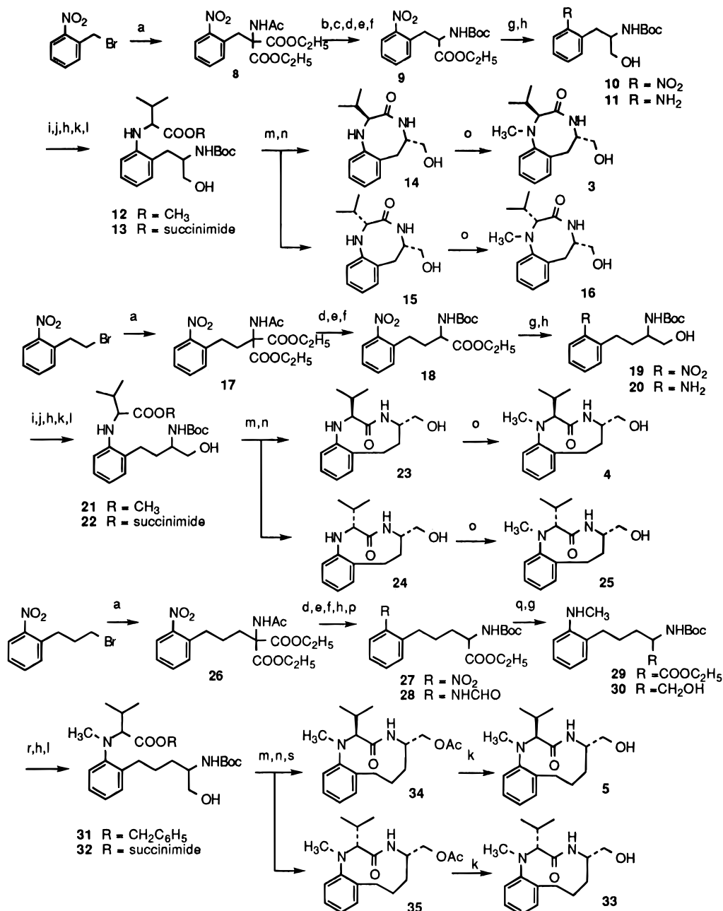
Figure 4. Synthesis of benzolactams (BL-V8: 3 , BL-V9: 4 and BL-V10: 5 ). Key: (a) \text{CH}_3\text{CONHCH}(\text{COOC}_2\text{H}_5)_2 , NaH/DMF; (b) KOH/ \text{H}_2\text{O} ; (c) HCl/ \text{H}_2\text{O} ; (d) HCl/AcOH; (e) \text{SOCl}_2 /EtOH; (f) \text{Boc}_2\text{O}/\text{CH}_2\text{Cl}_2 ; (g) \text{LiBH}_4 /THF; (h) \text{H}_2 , Pd-C/ \text{CH}_3\text{COOC}_2\text{H}_5 - \text{H}_2\text{O} ; (i) methyl 2-oxoisovalerate; (j) \text{NaBH}_3\text{CN} , THF; (k) KOH/ \text{CH}_3\text{OH} - \text{H}_2\text{O} ; (l) N -hydroxysuccinimide, DCC/ \text{CH}_3\text{CN} ; (m) \text{CF}_3\text{COOH}/\text{CH}_2\text{Cl}_2 ; (n) \text{NaHCO}_3(\text{aq})/\text{CH}_3\text{COOEt} ; (o) \text{CH}_3\text{I} , \text{NaHCO}_3/\text{CH}_3\text{OH} ; (p) \text{HCOOH} , \text{Ac}_2\text{O} ; (q) \text{BH}_3 /THF; (r) triflate of benzyl DL- \alpha -hydroxyisovalerate, 2,6-lutidine/ \text{CH}_2\text{ClCH}_2\text{Cl} ; (s) \text{Ac}_2\text{O} /pyridine.
