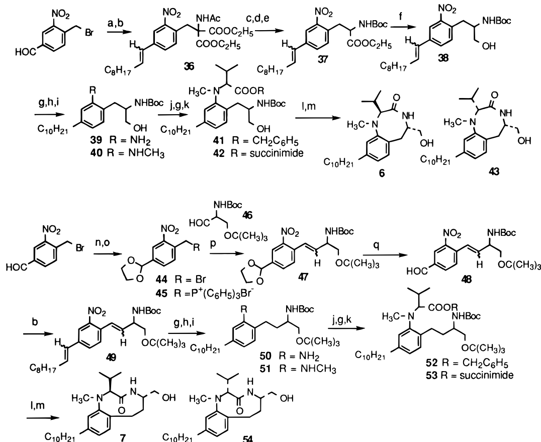
Figure 5. Synthesis of benzolactams (BL-V8-310: 6 and BL-V9-310: 7). Key: (a) \text{CH}_3\text{CONHCH}(\text{COOC}_2\text{H}_5)_2 , \text{NaH}/\text{DMF} ; (b) \text{C}_9\text{H}_{19}\text{P}^+\text{Ph}_3\text{Br}^- , n\text{-BuLi}/\text{THF} ; (c) \text{HCl}/\text{AcOH} ; (d) \text{SOCl}_2/\text{EtOH} ; (e) \text{Boc}_2\text{O}/\text{CH}_2\text{Cl}_2 ; (f) \text{LiBH}_4/\text{THF} ; (g) \text{H}_2 , \text{Pd}-\text{C}/\text{EtOH} ; (h) \text{HCOOH} , \text{Ac}_2\text{O} ; (i) \text{BH}_3/\text{THF} ; (j) triflate of benzyl DL- \alpha -hydroxyisovalerate, 2,6-lutidine/ \text{CH}_2\text{ClCH}_2\text{Cl} ; (k) N -hydroxysuccinimide, \text{DCC}/\text{CH}_3\text{CN} ; (l) \text{CF}_3\text{COOH}/\text{CH}_2\text{Cl}_2 ; (m) \text{NaHCO}_3(\text{aq})/\text{CH}_3\text{COOEt} ; (n) \text{HOCH}_2\text{CH}_2\text{OH} , \text{TsOH}/\text{toluene} ; (o) \text{PPh}_3/\text{toluene} ; (p) 46, \text{K}_2\text{CO}_3/\text{DMF} ; (q) pyridinium p -toluenesulfonate/acetone, \text{H}_2\text{O} .
