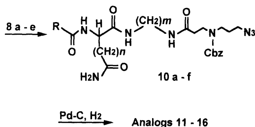
Chart 2. Coupling of Synthons
