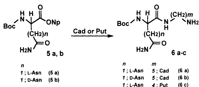
Chart 1. Preparation of Synthons I and II
