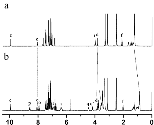
FIGURE 5. Partial ^1\text{H} NMR spectra (400 MHz, 1 \times 10^{-3} M, DMSO- d_6 ) of T-3 (a) and R-3 (b).
