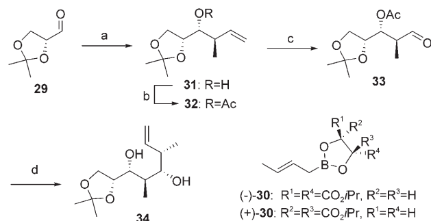
Scheme 4. Iterative crotyl addition reactions. a) (-)\text{-30} , 4 Å MS, toluene, -78^\circ\text{C} , 7 h, 65%; b) \text{Ac}_2\text{O} , \text{Et}_3\text{N} , DMAP (cat), \text{CH}_2\text{Cl}_2 , RT, overnight, 95%; c) \text{O}_3 , \text{MeOH} , -78^\circ\text{C} ; then \text{PPh}_3 , RT, 85%; d) (+)\text{-30} , 4 Å MS, toluene, -78^\circ\text{C} , 6 h, 70%.
