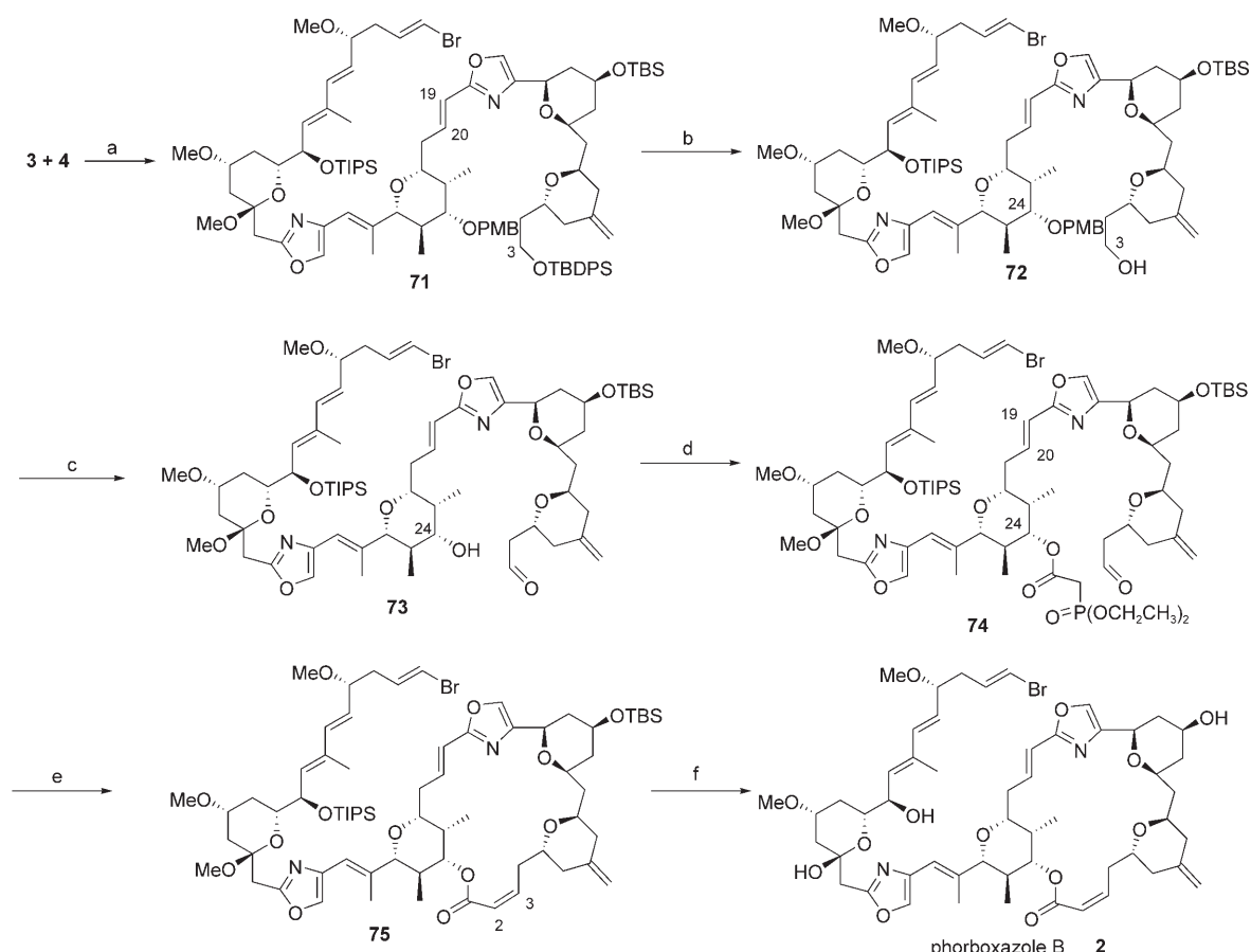
Scheme 10. Completion of the synthesis of phorboxazole B. a) \text{Bu}_3\text{P} , DMF; then 4 , DBU, RT, 70%; b) \text{NH}_4\text{F} , MeOH, 50^\circ\text{C} , 71%; c) 1) Dess–Martin periodinane, py, \text{CH}_2\text{Cl}_2 , RT; 2) DDQ, \text{CH}_2\text{Cl}_2 , buffer (pH 7), 73% for the two steps; d) dimethyl phosphonoacetic acid, DCC, \text{CH}_2\text{Cl}_2 , 85%; e) \text{K}_2\text{CO}_3 , [18]crown-6, toluene, -20^\circ\text{C} , Z/E 5:1, 67%; f) 1) TBAF, THF, RT; 2) 6% HCl, THF, 51% for the two steps.
