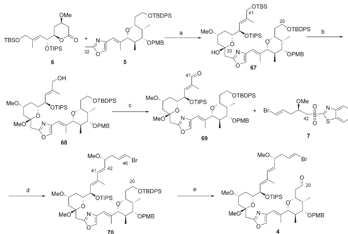
Scheme 9. Synthesis of the C20–C46 segment. a) \text{LiNEt}_2 , THF, -78^\circ\text{C} ; then 6 , 61 %; b) PPTS, MeOH, 30^\circ\text{C} , 81 %; c) Dess–Martin periodinane, py, \text{CH}_2\text{Cl}_2 , RT, 93 %; d) NaHMDS, THF, -78^\circ\text{C} , 78 %; e) 1) \text{NH}_4\text{F} , MeOH, 50^\circ\text{C} ; 2) Dess–Martin periodinane, py, \text{CH}_2\text{Cl}_2 , RT, 71 % for the two steps.
