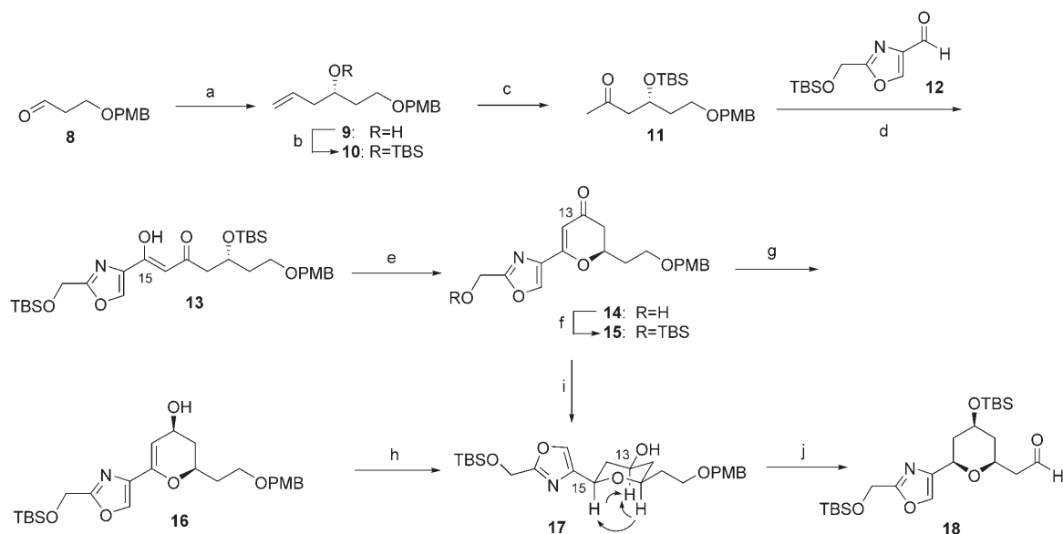
Scheme 2. Synthesis of the C9–C19 segment 18 . a) (–)-Ipc 2 Ballyl, Et 2 O, –78 °C, 87% ee , 71%; b) TBSCl, imidazole, DMF, 96%; c) PdCl 2 (cat), CuCl, O 2 , DMF/H 2 O, RT, 6 h, 89%; d) 1) LDA, 12 , THF, –78 °C; 2) Dess–Martin periodinane, CH 2 Cl 2 , RT, 90% for the two steps; e) 5% HF in CH 3 CN, RT, 12 h, 90%; f) TBSCl, imidazole, DMF, RT, 97%; g) NaBH 4 , CeCl 3 , MeOH, –78 °C, 95%; h) H 2 , 10% Pd/C, EtOAc, 8 h, 95%; i) H 2 , 10% Pd/C, EtOAc (saturated with 0.1 N HCl), 8 h, 65%; j) 1) TBSCl, imidazole, DMF, RT; 2) DDQ, CH 2 Cl 2 , RT; 3) Dess–Martin periodinane, CH 2 Cl 2 , RT, 82% for the three steps.
