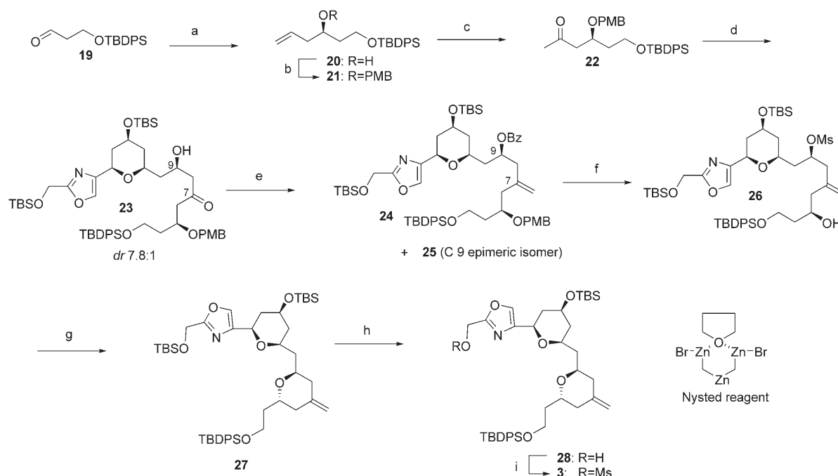
Scheme 3. Completion of the C3–C19 segment 3 . a) (+)-Ipc 2 BAllyl, Et 2 O, -78^{\circ}\text{C} , 87% ee , 74%; b) PMBOC(=NH)CCl 3 , cyclohexane/CH 2 Cl 2 , BF 3 ·OEt 2 , 0^{\circ}\text{C} , 87%; c) PdCl 2 (cat), CuCl, O 2 , DMF/H 2 O, RT, 6 h, 86%; d) 1) LHDMS, TMSCl, THF, -78^{\circ}\text{C} ; 2) 18 , TiCl 4 , -78^{\circ}\text{C} , 68%; e) 1) BzCl, py (pyridine), RT; 2) Nysted reagent, TiCl 4 , RT, 30 min, 66% for the two steps; f) 1) DIBAL, CH 2 Cl 2 , -78^{\circ}\text{C} ; 2) MsCl (Ms = mesyl), Et 3 N, CH 2 Cl 2 , 0^{\circ}\text{C} ; 3) DDQ, CH 2 Cl 2 /H 2 O, 67% for the three steps; g) Et 3 N, CH 3 CN, reflux, 83%; h) NH 4 F, MeOH, 50^{\circ}\text{C} , 81%; i) DIPEA, MsCl, 90%.
