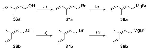
Scheme 9. Synthesis of Grignard reagent 38 . a) \text{PBr}_3 , pyridine, \text{Et}_2\text{O} , -30^\circ\text{C} , 30 min, 83% for 37a , 80% for 37b ; b) Mg, \text{Et}_2\text{O} , -10 \rightarrow -5^\circ\text{C} , 12 h.
