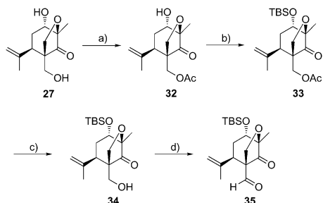
Scheme 8. Synthesis of keto-aldehyde 35 . a) AcCl, i\text{Pr}_2\text{EtN} , \text{CH}_2\text{Cl}_2 , 0^\circ\text{C} to rt, 4 h, 97%; b) TBDMSOTf, 2,6-lutidine, \text{CH}_2\text{Cl}_2 , rt, 2 h, 100%; c) NaOH, MeOH, THF, rt, 4 h, 96%; d) TPAP, NMO, \text{CH}_2\text{Cl}_2 , rt, 2 h, 84%.
