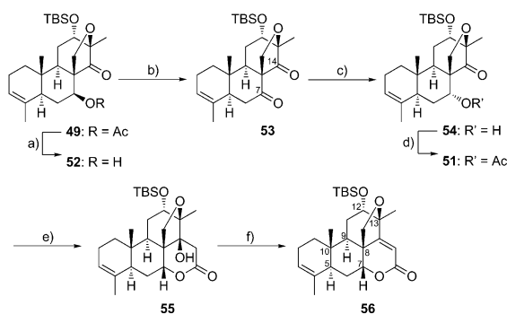
Scheme 16. Synthesis of \alpha,\beta -unsaturated lactone 56 a) \text{NaOH} , \text{MeOH} , rt, 12 h, 96%; b) Dess–Martin periodinane, \text{CH}_2\text{Cl}_2 , rt, 6 h, 96%; c) K-selectride, THF, rt, 20 min, 97%; d) \text{Ac}_2\text{O} , DMAP, \text{CH}_2\text{Cl}_2 , rt, 24 h, 100%; e) LDA, toluene/THF 2:1, -30^\circ\text{C} , 30 min, 87%; f) \text{SOCl}_2 , pyridine, \text{CH}_2\text{Cl}_2 , 0^\circ\text{C} to rt, 12 h, 90%.
