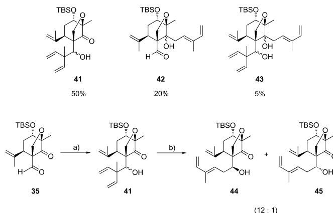
Scheme 11. Synthesis of IMDA precursor 44 and 45 . a) Grignard reagent 38 , \text{Et}_2\text{O} , rt, 5 min, 80%; b) KH, dibenzo-[18]crown-6, THF, rt, 4 h, 85%.
