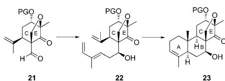
Scheme 6. Synthetic approach towards ABCE ring system.
