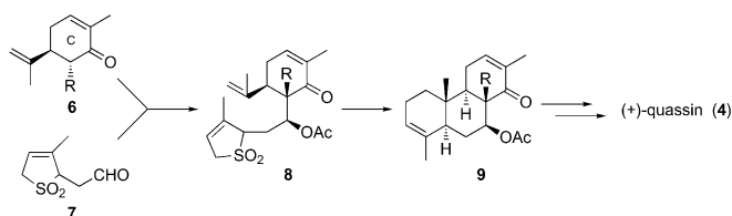
Scheme 2. Synthesis of quassin.
