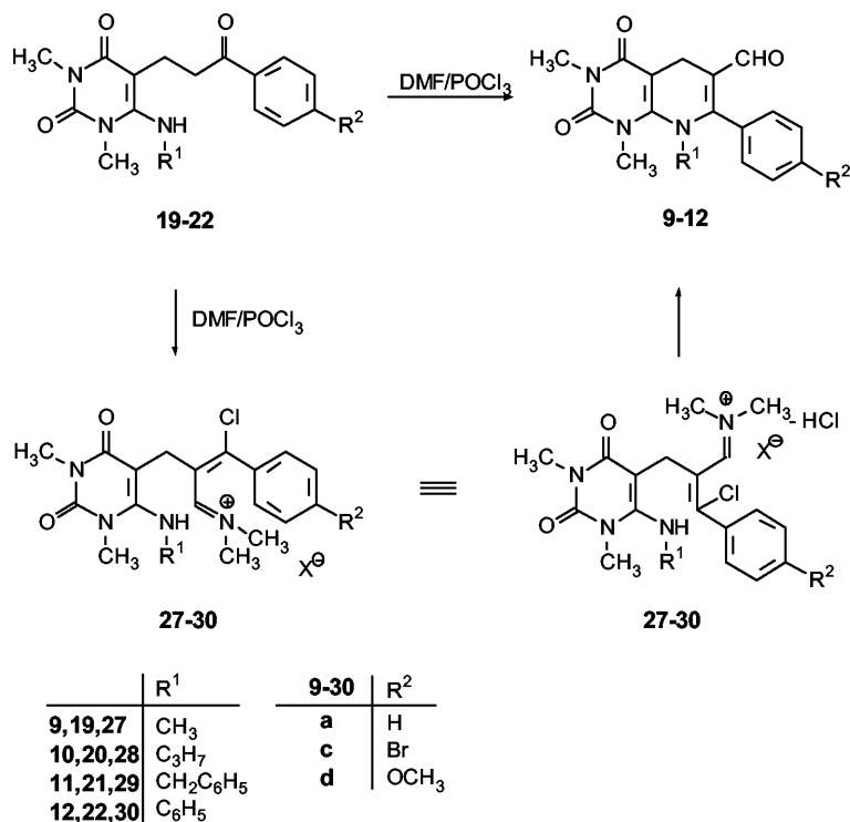
Scheme 6. Projected cyclization of the uracils 15 – 18 using ketone Mannich bases 2 .
