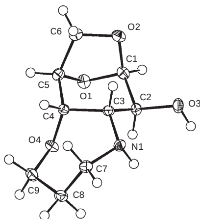
FIG. 1 View of compound 6 . Thermal ellipsoids are drawn on the 50% probability level (PLATON 8 )
