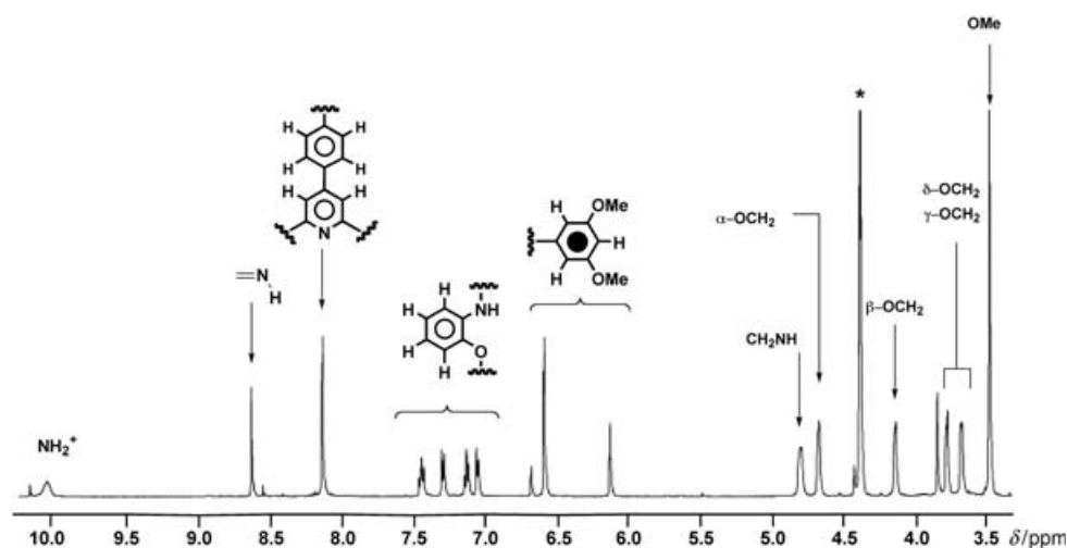
Figure 7. Partial ^1\text{H} NMR spectrum (500 MHz) of the dynamic bis[2]rotaxane prior to the reduction of the imine bonds ( \alpha , \beta , \gamma , \delta -OCH _2 correspond to the protons of the ethylene glycol chain as labeled in Scheme 3).
