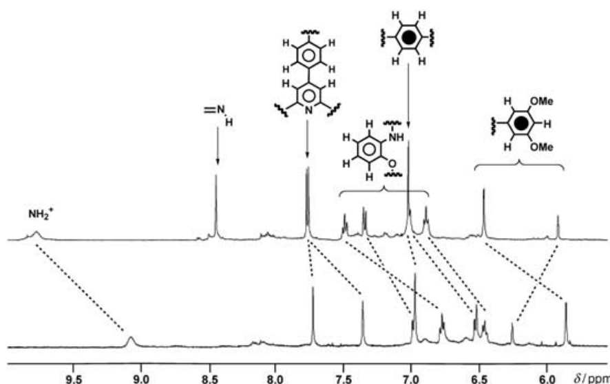
Figure 9. Partial ^1H NMR spectra (500 MHz, CD_3NO_2 ) of the dynamic cyclic [4]rotaxane formation (upper trace) and of its related kinetically stable cyclic [4]rotaxane [18-H_4][PF_6]_4 (lower trace) after reduction of the imine bonds.
