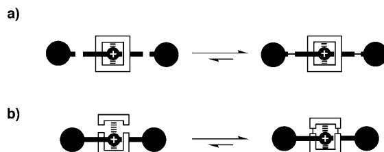
Figure 1. Formation of a [2]rotaxane a) by a dynamic-stoppering and b) by a dynamic-clipping approach.
